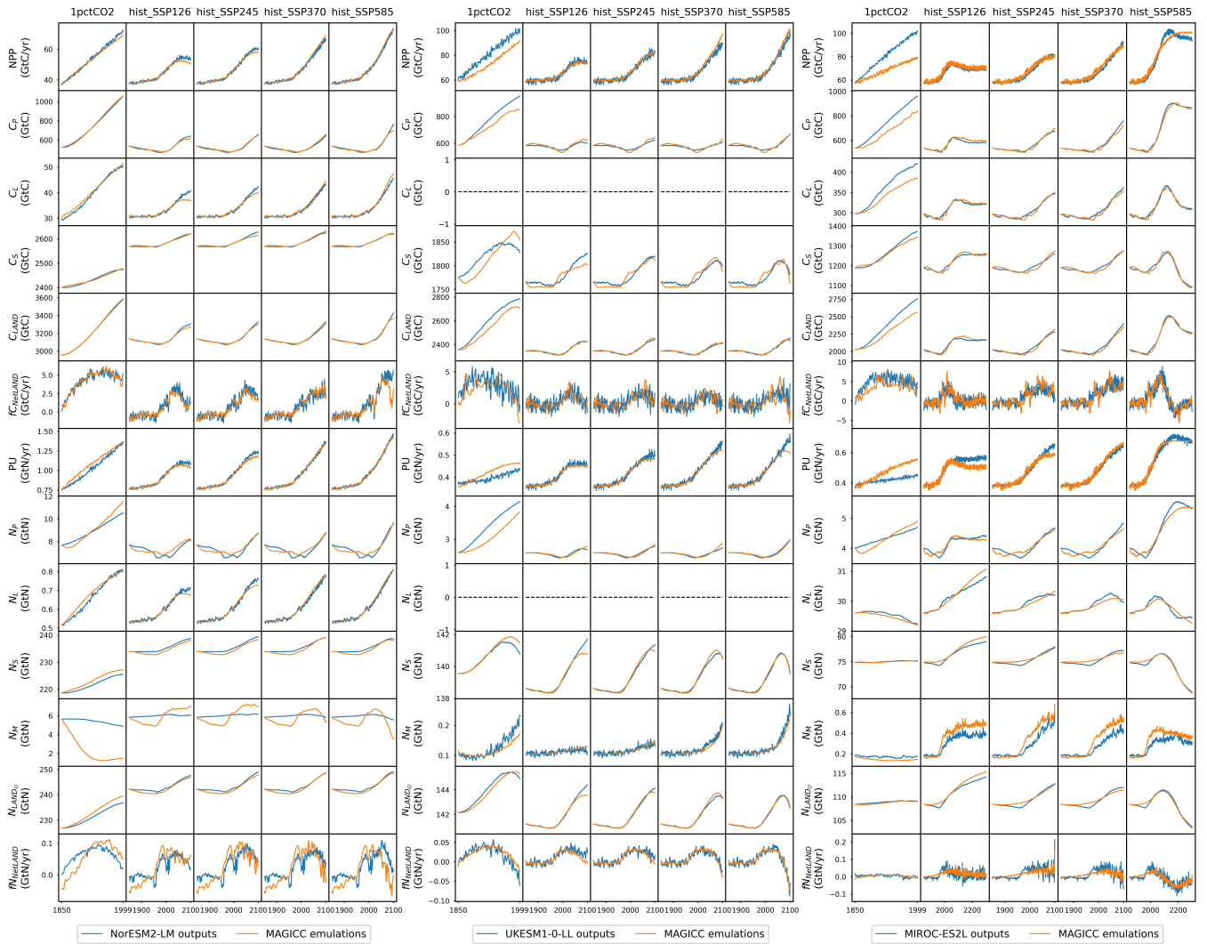
Figure A6. Comparison of ‘net primary production’ (NPP), ‘plant carbon pool size’ ( C_P ), ‘litter carbon pool size’ ( C_L ), ‘soil carbon pool size’ ( C_S ), ‘land carbon pool size’ ( C_{LAND} ), ‘net land carbon flux’ ( fC_{NetLAND} ), ‘nitrogen plant uptake’ (PU), ‘plant nitrogen pool size’ ( N_P ), ‘litter nitrogen pool size’ ( N_L ), ‘soil nitrogen pool size’ ( N_S ), ‘mineral nitrogen pool size’ ( N_M ), ‘land organic nitrogen pool size’ ( N_{LAND_o} , sum of nitrogen in plant, litter, and soil pools), and ‘net land nitrogen flux’ ( fN_{NetLAND} ) between CMIP6 ESM outputs (blue lines) and CNit emulations (orange lines).
