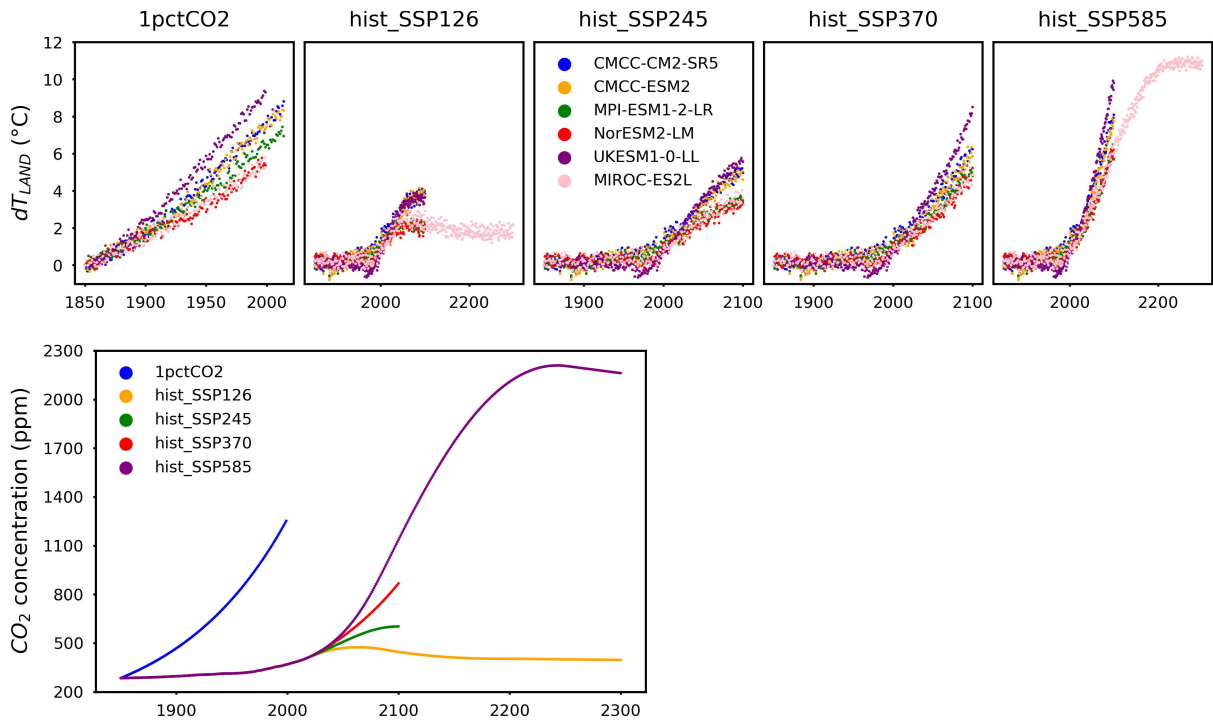
890 Figure A4. Global average 'surface temperature change over land' ( dT_{LAND} , delta annual mean tas over land) and \text{CO}_2 concentrations from CMIP6 ESMs across different scenarios.
