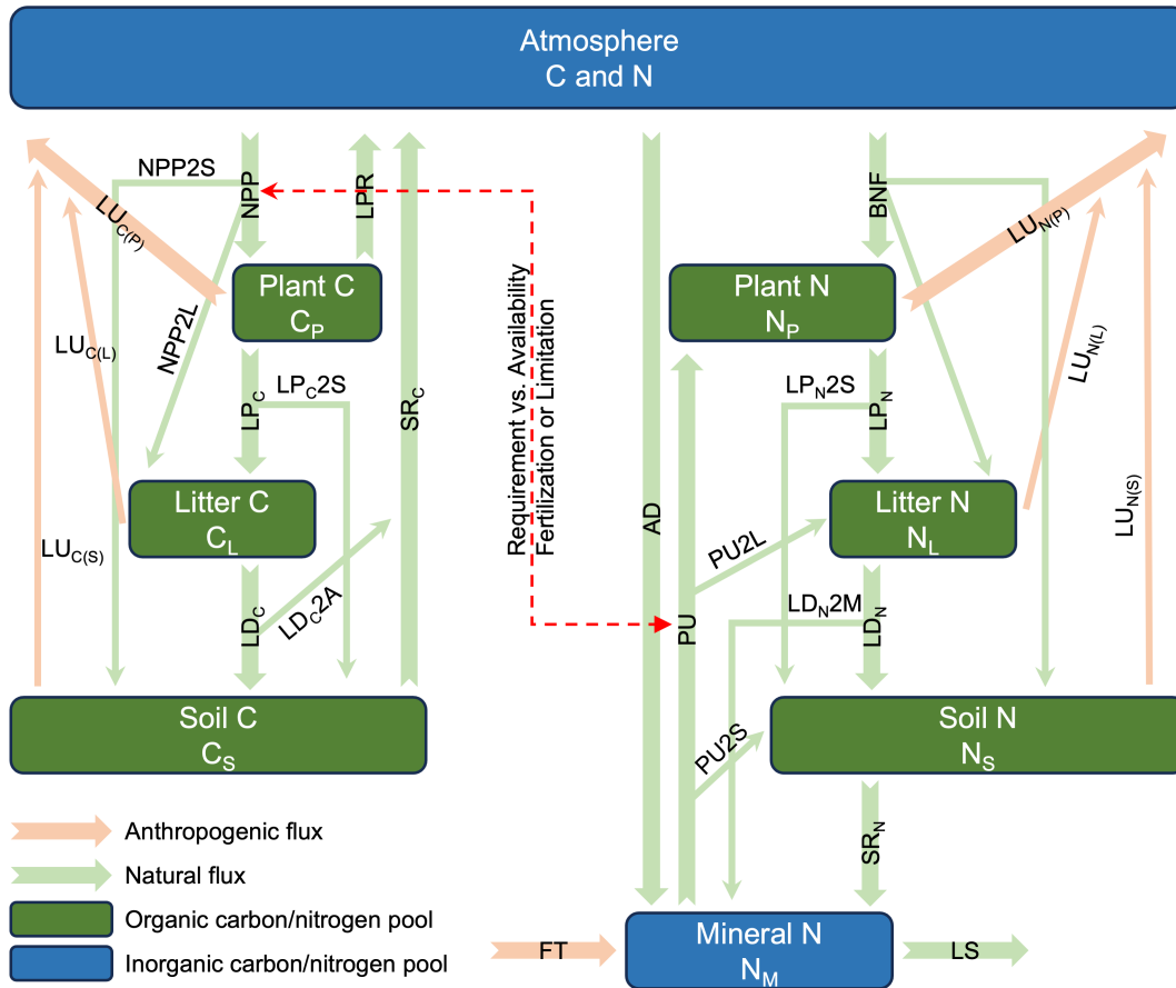
Figure 1. The ‘coupled carbon-nitrogen cycle’ (CNit) model in MAGICC (NPP: net primary production, LPR: litter production respiration, PU: nitrogen plant uptake, BNF: biological nitrogen fixation, LP: litter production, LD: litter decomposition, SR: soil respiration, LS: mineral nitrogen loss, LU: land use emission, AD: atmosphere nitrogen deposition, FT: nitrogen fertilizer application, 2P, 2L, 2S, and 2M: the partition of fluxes into plant, litter, soil, and mineral pools). The carbon and nitrogen mass conservation is described in Section 2.2. The NPP simulation is described in Section 2.3. The carbon-nitrogen coupling is described in Section 2.4. The LPR flux is described in Section 2.5. Each pool’s turnover time and its response to climate and carbon-nitrogen coupling are described in Section 2.6. The land use emission parameterisation is described in Section 2.7.
