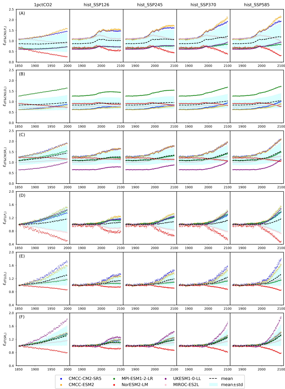
975 Figure A10. The emulated overall and temperature effect on carbon pool turnovers, including litter production ( \epsilon_{dT\&CN(LP_c)} and \epsilon_{dT(LP_c)} ), litter decomposition ( \epsilon_{dT\&CN(LD_c)} and \epsilon_{dT(LD_c)} ), and soil respiration ( \epsilon_{dT\&CN(SR_c)} and \epsilon_{dT(SR_c)} ) from CMIP6 ESMs across different scenarios.
