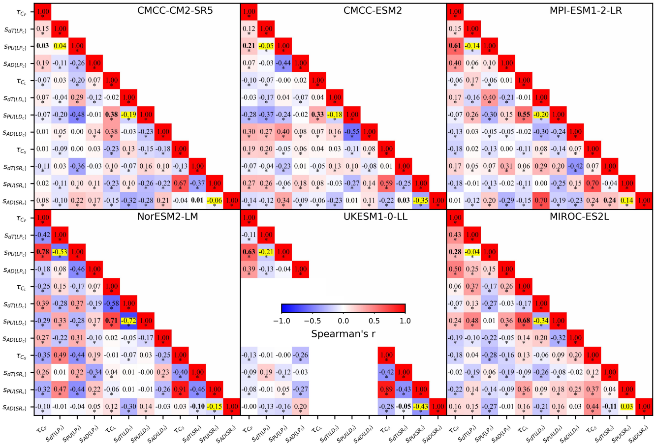
Figure A9. Correlation of turnover times and feedback-related parameters from the CMIP6 ESMs. The numbers indicate Spearman's correlation coefficients (r) between pairs of parameters, with * denoting p-values < 0.001. Correlations between temperature sensitivities and plant nitrogen uptake sensitivities are highlighted in yellow, while correlations between turnover times and plant nitrogen uptake sensitivities are shown in bold. Missing values for UKESM1-0-LL are due to the absence of a litter pool in this model, resulting in no turnover time or feedback-related parameters for the litter pool.
