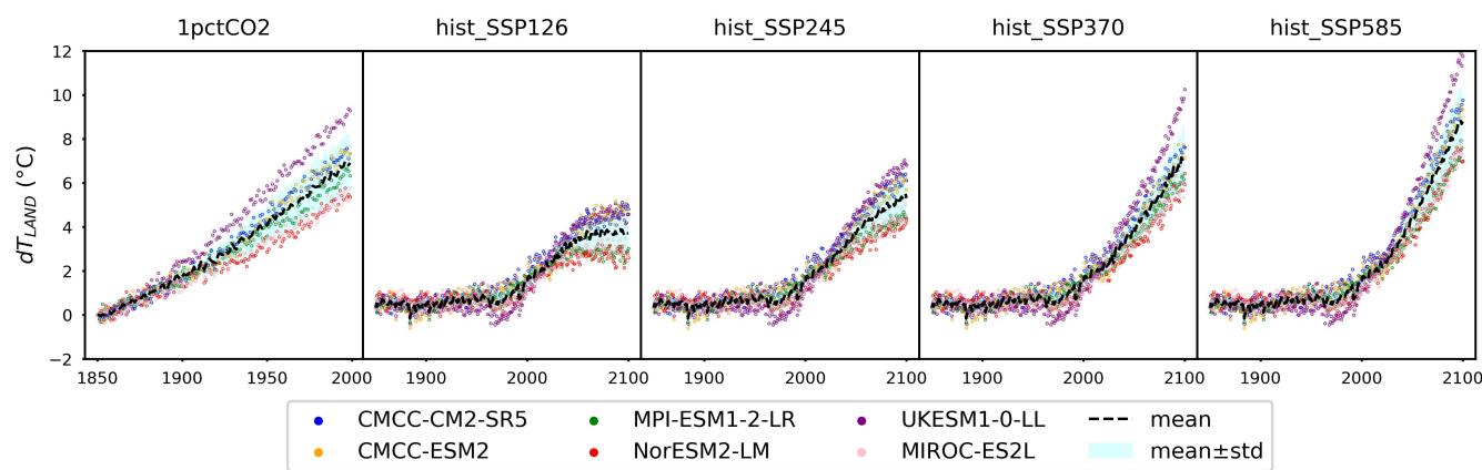
925 Figure A7. Global average ‘surface temperature change over land’ ( dT_{LAND} , delta annual mean tas over land) from CMIP6 ESMs across different scenarios (over the common experimental period).
