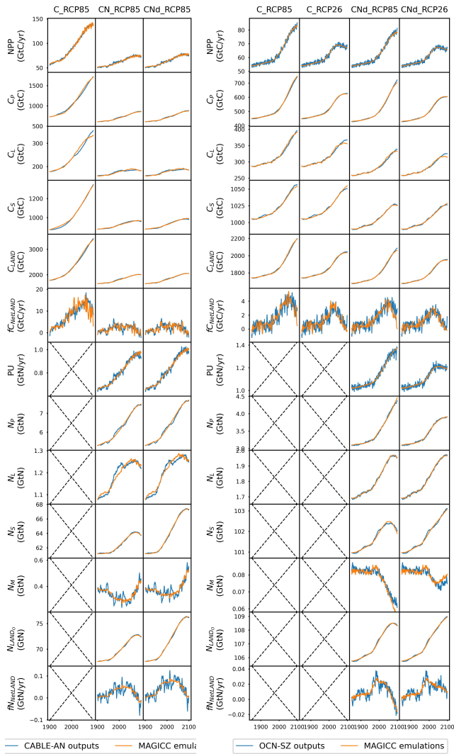
Figure A5. Comparison of ‘net primary production’ (NPP), ‘plant carbon pool size’ ( C_p ), ‘litter carbon pool size’ ( C_l ), ‘soil carbon pool size’ ( C_s ), ‘land carbon pool size’ ( C_{\text{LAND}} ), ‘net land carbon flux’ ( fC_{\text{NetLAND}} ), ‘nitrogen plant uptake’ (PU), ‘plant nitrogen pool size’ ( N_p ), ‘litter nitrogen pool size’ ( N_l ), ‘soil nitrogen pool size’ ( N_s ), ‘mineral nitrogen pool size’ ( N_m ), ‘land organic nitrogen pool size’ ( N_{\text{LAND}_o} , sum of nitrogen in plant, litter, and soil pools), and ‘net land nitrogen flux’ ( fN_{\text{NetLAND}} ) between CABLE or OCN outputs (blue lines) and CNit emulations (orange lines). The experiments labeled as C, CN, and CNd denote the carbon-only, carbon-nitrogen coupled with constant nitrogen atmospheric deposition, and carbon-nitrogen coupled with dynamic nitrogen atmospheric deposition configurations in the land surface models, respectively.
