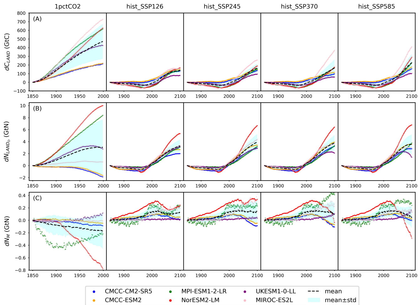
595 Figure 4. Carbon and nitrogen pool size dynamics [ dC_{LAND} , delta land carbon pool size; dN_{LAND_o} , delta land organic nitrogen pool size (sum of nitrogen in plant, litter, and soil pools); dN_M , delta mineral nitrogen pool size] from CMIP6 ESMs across different scenarios.
