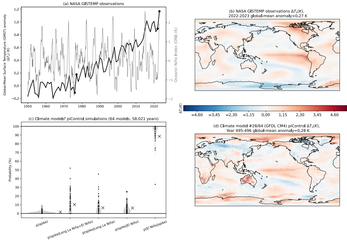
100 Figure 1: a. Annual-mean global-mean surface temperature (GMST) anomalies (baseline 1951-1980; black) and monthly-mean Oceanic Niño Index (detrended; grey) from NASA GISTEMP observations. Dots represent GMST spikes ( \Delta GMST > 0.25 K) from 1976 to 1977 and 2022 to 2023. b. Spatial pattern of surface temperature change from 2022 to 2023, i.e., 2023 spike, from NASA GISTEMP observations. c. Probabilities based on Eq. (A1) - (A5). Dots denote each model and crosses denote the multi-model mean (MMM). d. Spatial pattern of a surface temperature change from Year 495 to Year 496 in one of the 64 models' piControl simulations analyzed (GFDL CM4) is provided as an example.
