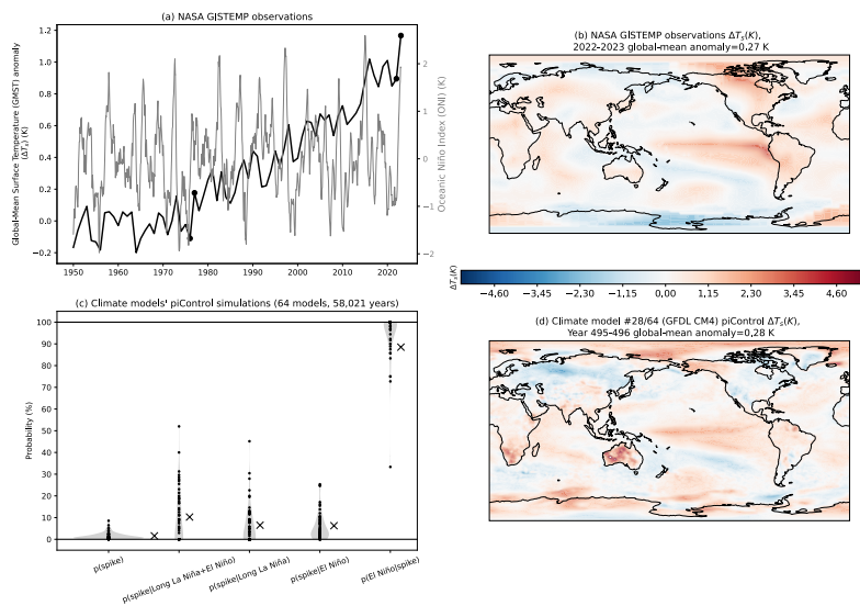
Figure 1: a. Annual-mean global-mean surface temperature (GMST) anomalies (baseline 1951-1980; black) and monthly-mean Oceanic Niño Index (detrended; grey) from NASA GISTEMP observations. Dots represent GMST spikes ( \Delta GMST > 0.25 K) from 1976 to 1977 and 2022 to 2023. b. Spatial pattern of surface temperature change from 2022 to 2023, i.e., 2023 spike, from NASA GISTEMP observations. c. Probabilities based on Eq. (A1) - (A5). Dots denote each model and crosses denote the multi-model mean (MMM). d. Spatial pattern of a surface temperature change from Year 495 to Year 496 in one of the 64 models' piControl simulations analyzed (GFDL CM4) is provided as an example.
