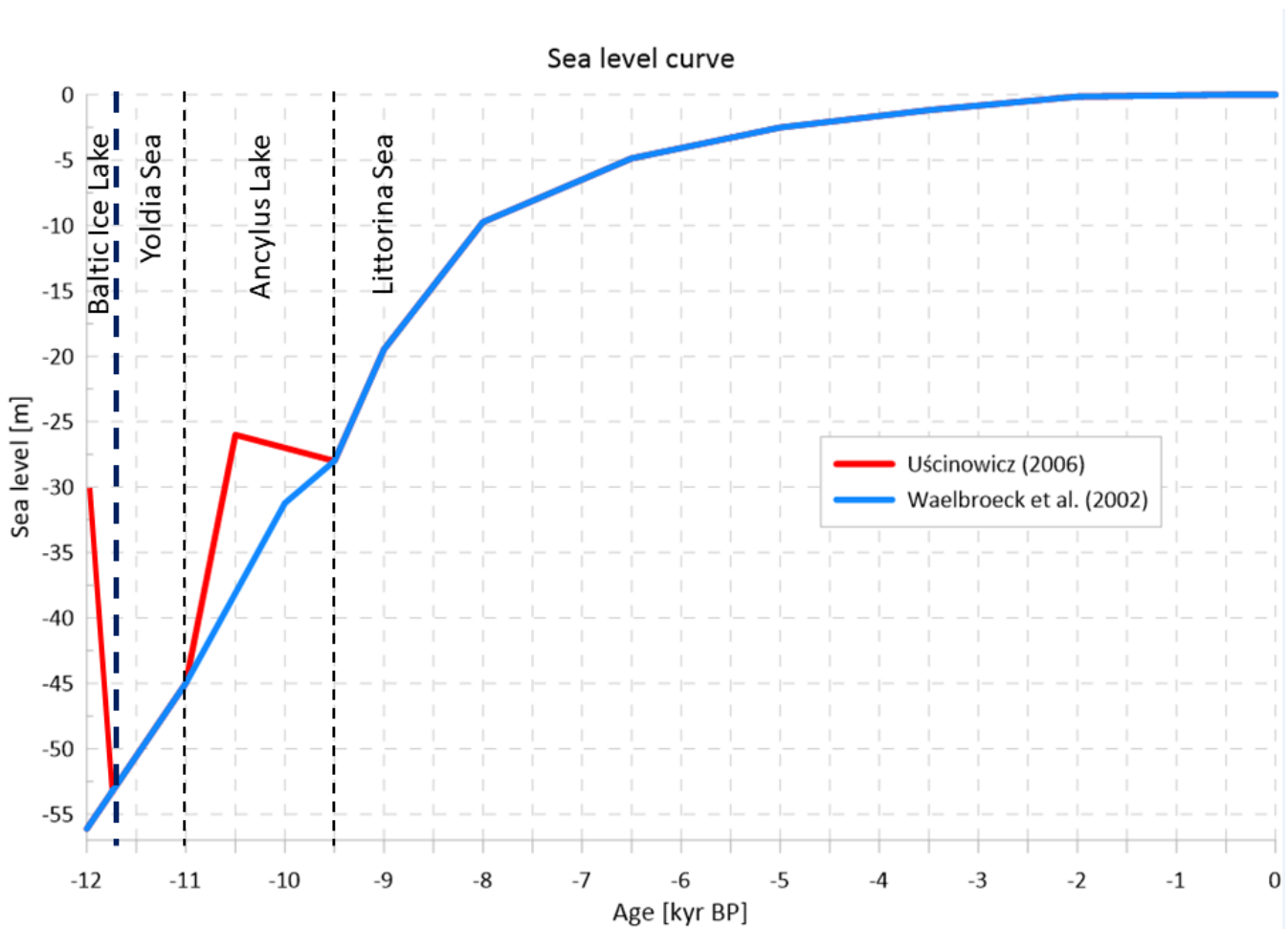
180 Figure 3: Holocene water level curve for the Baltic region generated by combination of Waelbroeck et al. (2002) and 185 Ućcinowicz (2006).
