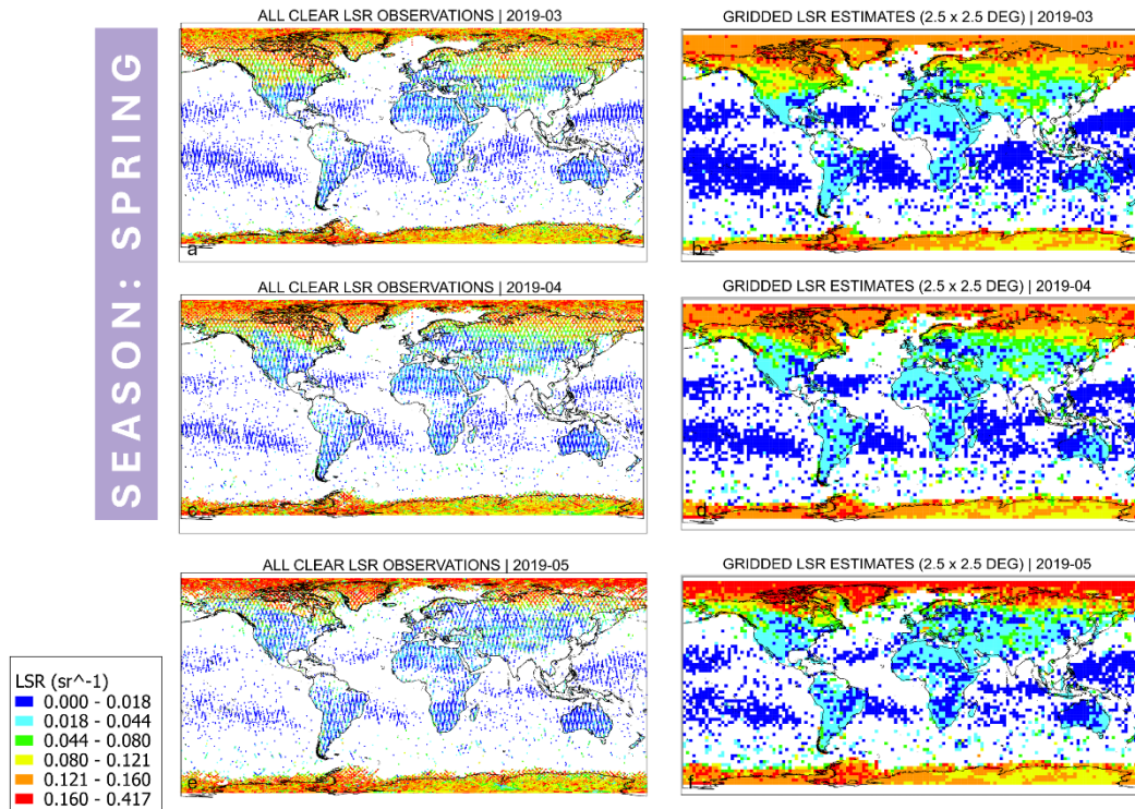
560 Fig 12. Panels a, c, e: all clear (qflag = 0, AOD < 1.0) LSR observations for March, April and May 2019, respectively. Panels b, d, f, gridded LSR estimates at 2.5° x 2.5° resolution based on the observations from the left for same months
