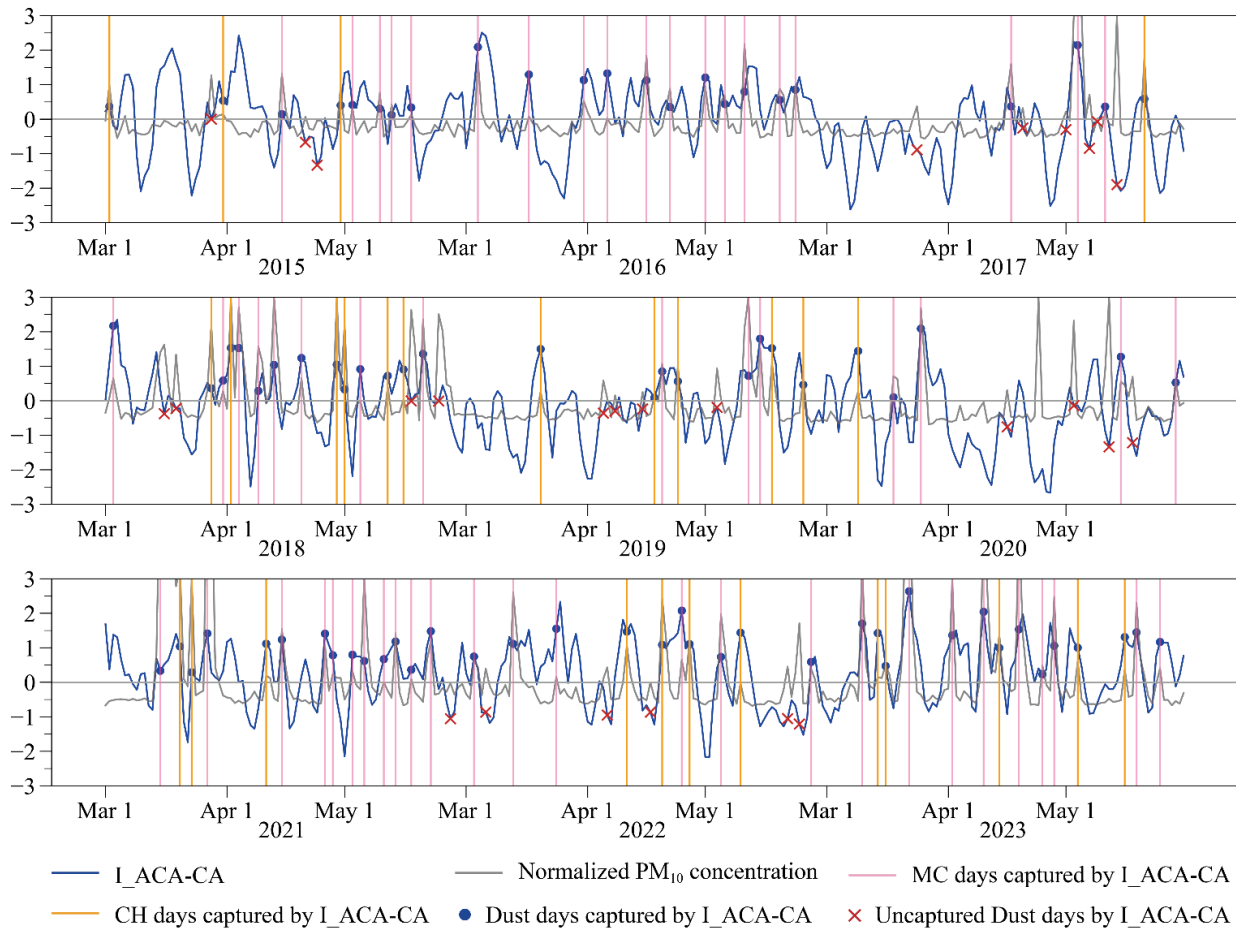
290 Figure 6. Daily I_ACA-CA (blue line) and normalized daily maximum PM 10 concentrations observed in NC (grey line) in March (Mar), April (Apr) and May from 2015 to 2023. The blue dots indicate the Dust days captured when I_ACA-CA > 0 and the corresponding I_ACA- CA value. The pink and yellow vertical lines indicate the MC days and CH days captured when I_ACA-CA > 0, respectively. The red "x" marks represent the Dust days that I_ACA-CA failed to capture.
