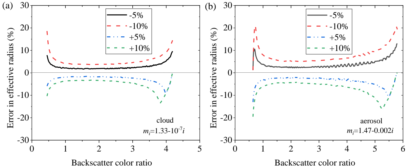
250 251 Figure 7. Errors in effective radius in Look-Up-Table when there are \pm 5\% and \pm 10\% errors in the backscatter color ratio. (a) Cloud 252 droplets, (b) aerosol particles.
