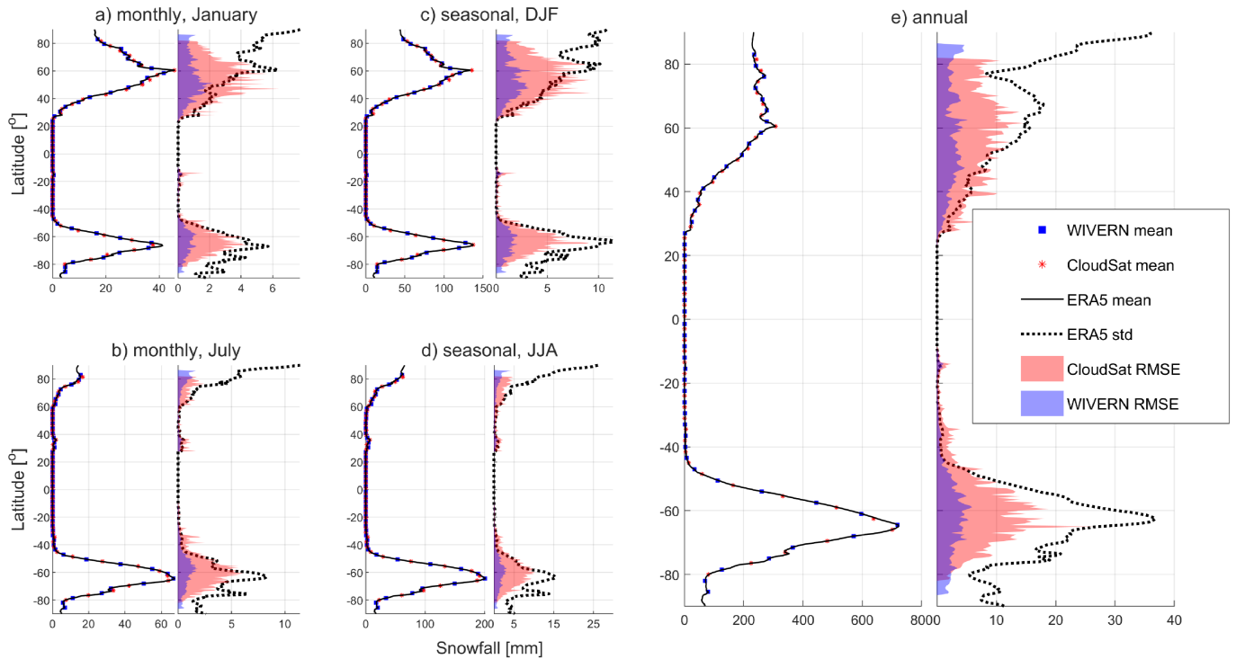
Figure 6. The figure shows the zonal mean snowfall at the monthly (January in panel a , and July in panel b ), seasonal (DJF in panel c , and JJA in panel d ) and annual (in panel e ) timescales. The ERA5, WIVERN and CloudSat mean value are depicted with a solid black line, blue markers and red markers, respectively. The inter-annual variability of the zonal mean (i.e. ERA5 standard deviation) is shown by the black dashed line. The shaded areas outline the RMSE of WIVERN and CloudSat.
