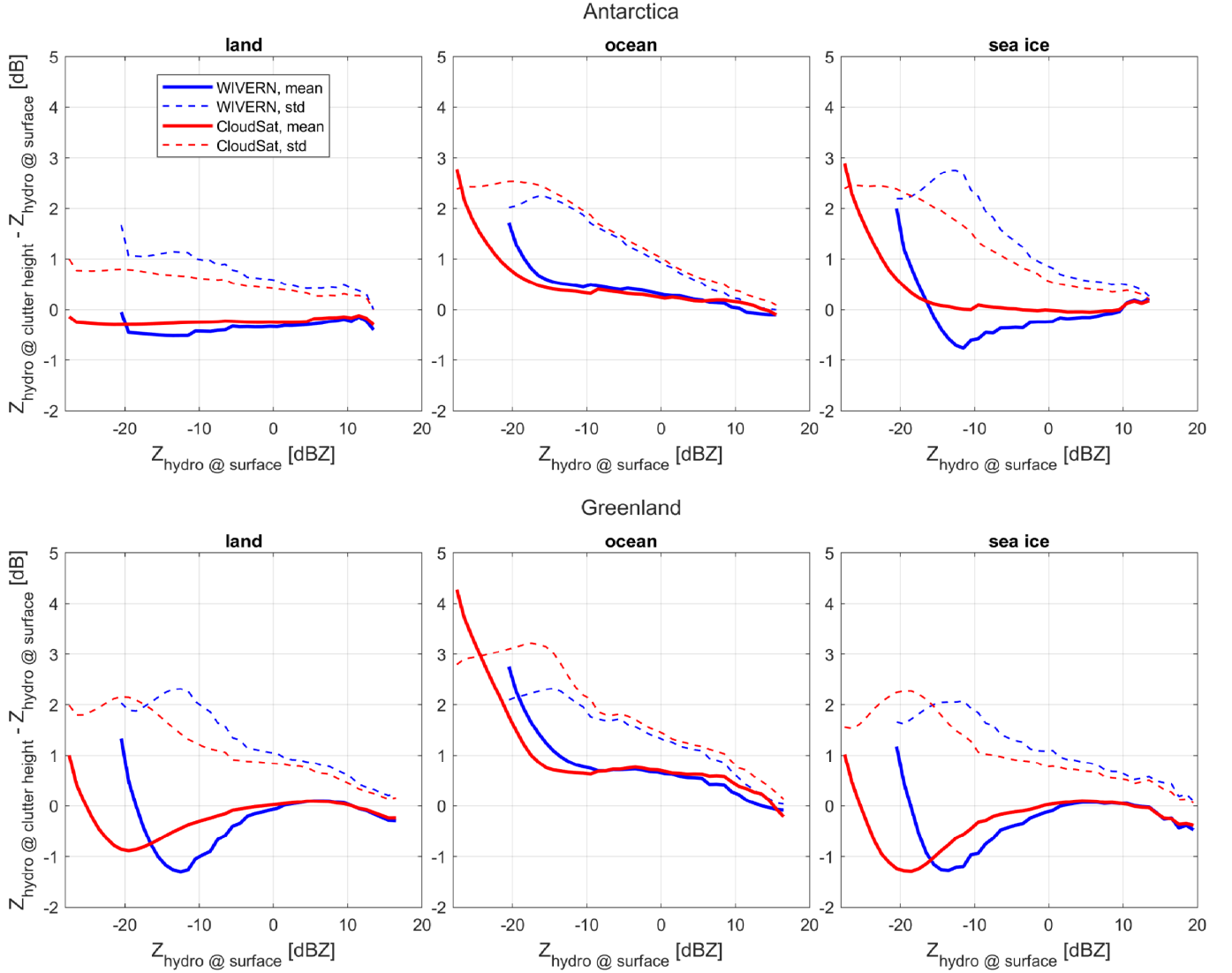
Figure 12. Mean (solid lines) and standard deviation (dashed lines) values of Z_{e,surf}^{hydro} - Z_{e,SCR=5dB}^{hydro} as a function of Z_{e,surf}^{hydro} , for WIVERN (blue) and CloudSat (red) for two different regions (top: Antarctica; bottom: Greenland) and three different surface types (left:land; centre: ice-free ocean; right:sea ice).
