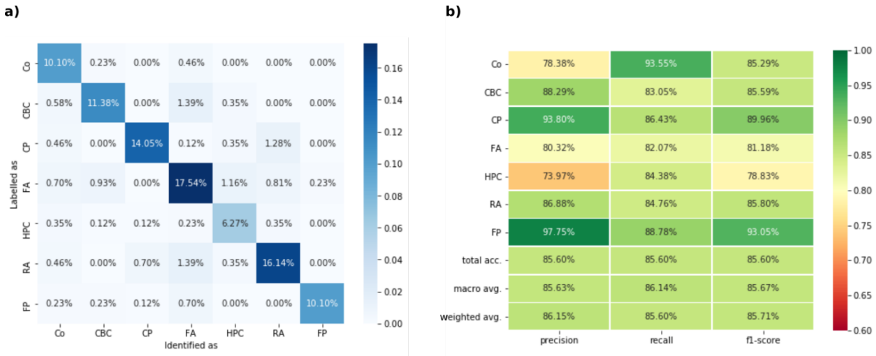
Figure 4. a) Confusion matrix for the HVPS CNN. b) Training report for the HVPS CNN.
