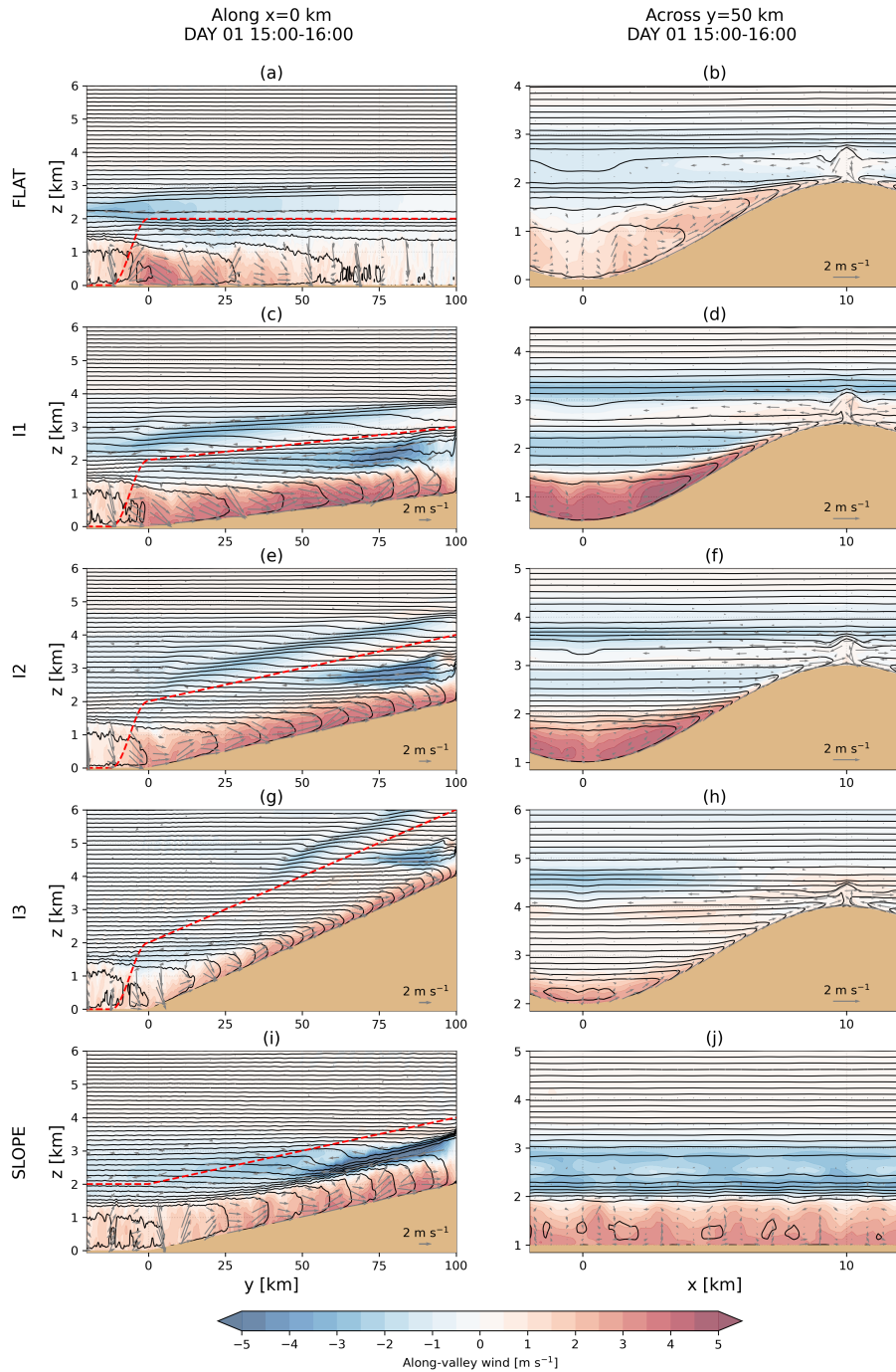
Figure 3. Vertical cross-sections along the domain centers at x = 0 km on the left column (panels a,c,e,g,i) and across the domain at y = 50 km on the right column (panels b,d,f,h,j). For all panels the along-valley wind is shaded (positive for up-valley wind, 0.5 \text{ m s}^{-1} interval) and potential temperature is plotted on contours ( 0.5 \text{ K} interval). Grey vectors show the wind component in the plotted plane. The plotted values are an hourly average of 15:00–16:00 on the first day of the simulation.
