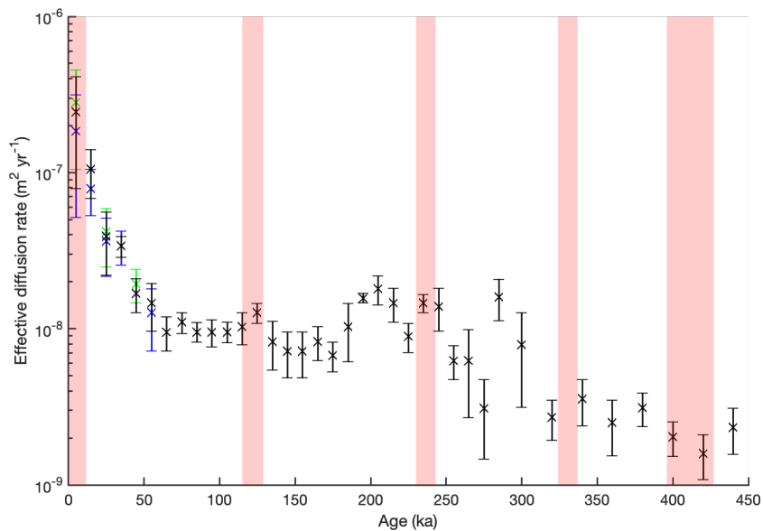
295 Figure 3: Effective diffusion rates of sulfate in the EDC core. For each time bin, the median (black crosses) and median absolute deviation (MAD, black vertical bars) of effective diffusion rates across all volcanic events are shown. For the first 6 time bins, median and MAD of effective diffusion rates are also shown for volcanic peaks with FWTM of 1 yr (green) and 5 yr (blue). Varying peak width has a negligible impact on results from older time bins. Time bins are 10 kyr duration except those >300 ka, which are 20 kyr in duration. Light red shaded regions denote interglacial periods.
