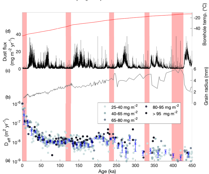
365 Figure 5: Effective diffusion rate estimated for each EDC volcanic sulfate peaks compared to grain size and dust loading. (a) Effective diffusion coefficient ( D_{\text{eff}} ) estimated for each individual volcanic sulfate peak, colour-coded according to magnitude of total sulfate flux (see legend). Median D_{\text{eff}} values and MAD range for each time bin are also plotted (blue crosses and vertical bars, as Fig. 3). (b) EDC grain radius (EPICA community members, 2004). (c) EDC dust flux (Lambert et al., 2008). (d) EDC borehole temperature profile (Buizert et al., 2021). Light red shaded regions denote interglacial periods.
