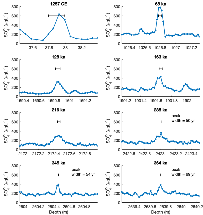
Figure 1: Selected volcanic sulfate peaks in the EDC ice core showing changes in peak shape with depth. All peaks shown have a total sulfate flux of 63.7–91.0 \text{mg m}^{-2} and in each case the x-axis spans a depth range of 1 m and the y-axis has the same scaling. The horizontal black bar on each plot indicates the depth range equivalent to 5 yr of accumulation at that depth in the core.
