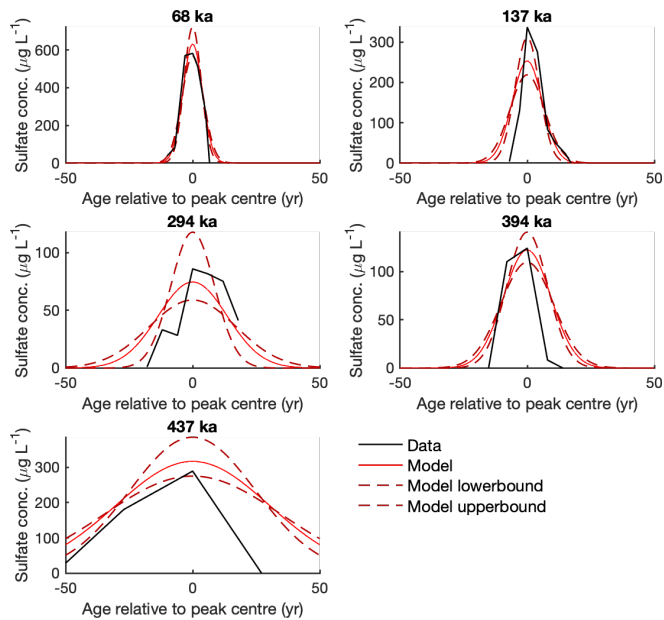
315 Figure 4: Comparison of sulfate peaks in ice core with peaks produced by forward model. EDC sulfate peaks (black) of different age (indicated by bold titles) are compared to forward model simulations (red) produced using the median effective diffusion rate for 10 kyr time bin (or 20 kyr time bin if peak age >300 ka). Model upper- and lower-bounds (dashed dark red) are product of the median \pm MAD effective diffusion rate (as Fig. 3).
