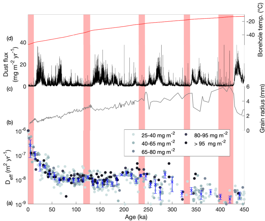
605 Figure 5: Effective diffusion rate estimated for each EDC volcanic sulfate peaks compared to grain size and dust loading. (a) Effective diffusion coefficient ( D_{\text{eff}} ) estimated for each individual volcanic sulfate peak, colour-coded according to magnitude of total sulfate flux (see legend). Median D_{\text{eff}} values and MAD range for each time bin are also plotted (blue crosses and vertical bars, as Fig. 3). (b) EDC grain radius (EPICA community members, 2004). (c) EDC dust flux (Lambert et al., 2008). (d) EDC borehole temperature profile (Buizert et al., 2021). Light red shaded regions denote interglacial periods.
