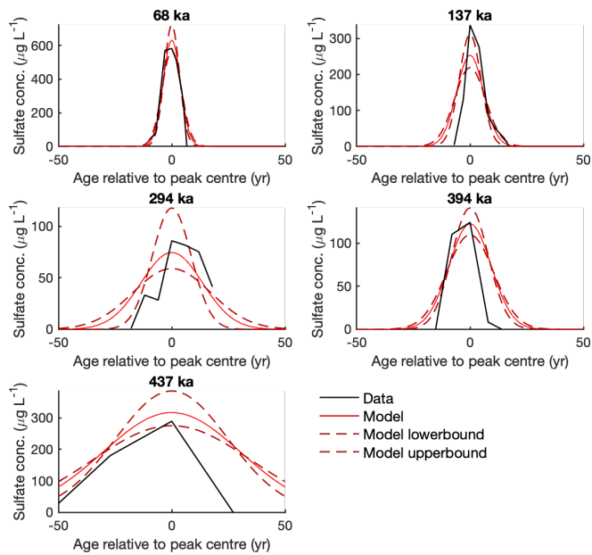
545 Figure 4: Comparison of sulfate peaks in ice core with peaks produced by forward model. EDC sulfate peaks (black) of different age (indicated by bold titles) are compared to forward model simulations (red) produced using the median effective diffusion rate for 10 kyr time bin (or 20 kyr time bin if peak age >300 ka). Model upper- and lower-bounds (dashed dark red) are product of the median \pm MAD effective diffusion rate (as Fig. 3).
