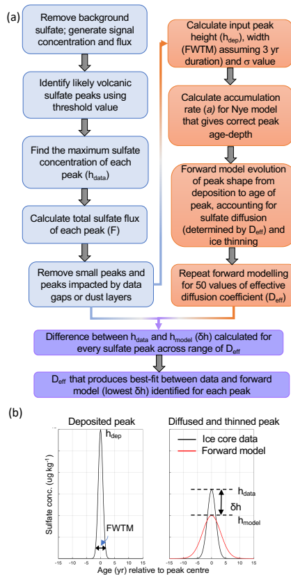
245 Figure 2: Illustration of methodology. (a) Flow chart of methodology involving analysis of EDC sulfate data (blue boxes), generation of equivalent deposited peaks and forward modelling (orange boxes), and data-model comparison to find effective diffusion coefficient (purple boxes); (b) Example of a sulfate peak preserved in the ice core (right-hand side, black curve), its equivalent deposited peak (left-hand side), and a peak produced by the forward model (right-hand side, red curve). In this example, the forward 250 model produces a peak that is lower in amplitude and broader than the ice core data peak, suggesting that the effective diffusion coefficient used was too high. Key parameters defined in the text are labelled.
