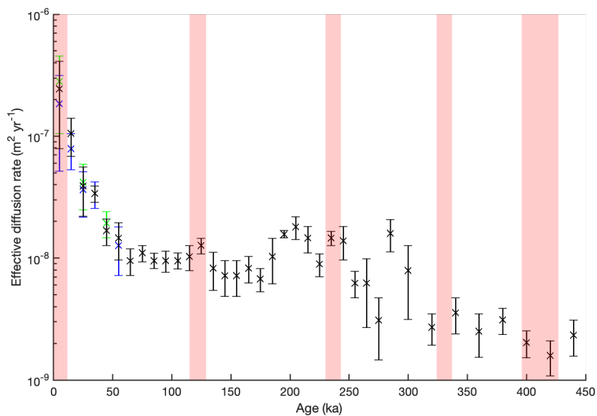
525 Figure 3: Effective diffusion rates of sulfate in the EDC core. For each time bin, the median (black crosses) and median absolute deviation (MAD, black vertical bars) of effective diffusion rates across all volcanic events are shown. For the first 6 time bins, median and MAD of effective diffusion rates are also shown for volcanic peaks with FWTM of 1 yr (green) and 5 yr (blue). Varying peak width has a negligible impact on results from older time bins. Time bins are 10 kyr duration except those >300 ka, which are 20 kyr in duration. Light red shaded regions denote interglacial periods.
