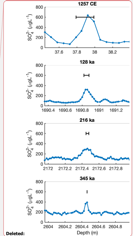
Figure 1: Selected volcanic sulfate peaks in the EDC ice core showing changes in peak shape with depth. All peaks shown have a total sulfate flux of 63.7–91.0 mg m -2 and in each case the x-axis spans a depth range of 1 m and the y-axis has the same scaling. The horizontal black bar on each plot indicates the depth range equivalent to 5 yr of ice accumulation at that depth in the core.
