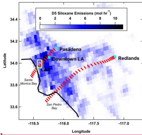
Figure 1: Example FLEXPART back-trajectory paths initiated in Pasadena or Redlands, CA. Red dashes indicate the particle cluster center-of-mass location at 15-minute intervals overlaid with 4 km spatial grids colored by hourly D5-siloxane emission rates from the FIVE-VCP-NEI17NRT inventory. An example model area boundary (8 × 8 km perimeter) used to extract emissions for a single model step is shown in yellow.
