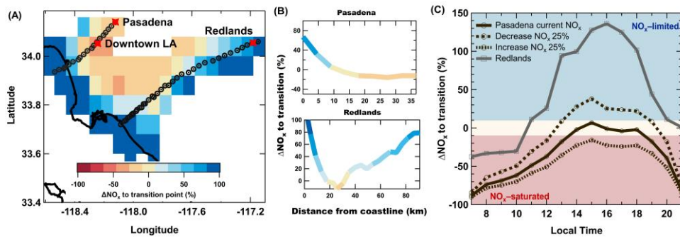
Figure 5: (A) The \text{NO}_x emissions required to reach the transition between chemical regimes ( \Delta\text{NO}_x(\text{transition}) ) averaged in 8 \times 8 km grids for times between 12:00-20:00 LT (%), only where n > 50 . Warmer colors (-%) indicate the location is currently \text{NO}_x -saturated, cooler (+%) is \text{NO}_x -limited, and neutral (pale yellow) indicates nearing the transitional regime ( \Delta\text{NO}_x(\text{transition}) = \pm 10\% ). The average trajectory path to Pasadena and Redlands is indicated by black markers. (B) The average \text{NO}_x emissions required to reach the transition within \pm 8 km of each average trajectory path is shown in Fig. 5B as a function of distance from the coastline (km) to Pasadena (top middle) and Redlands (bottom middle). (C) The predicted average (solid line) change in \text{NO}_x needed to transition between photochemical \text{O}_3 chemical regimes for the month of August, 2021 in Pasadena, CA. Red shading designates the current chemical regime as \text{NO}_x -saturated, blue shading designates \text{NO}_x -limited. The dashed lines simulate the sensitivity as the base case \text{NO}_x is increased and reduced by 25%. The solid grey line designates sensitivity results in Redlands, CA.
