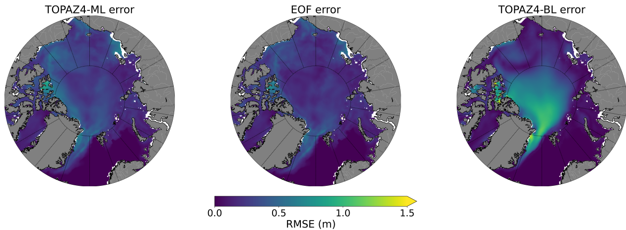
Figure 5. RMSE of SIT bias (m) over the test period (2011-2013) of left ) ML-adjusted error, middle ) EOF error, right ) baseline error against the SIT bias between TOPAZ4-FR and TOPAZ4-RA.
