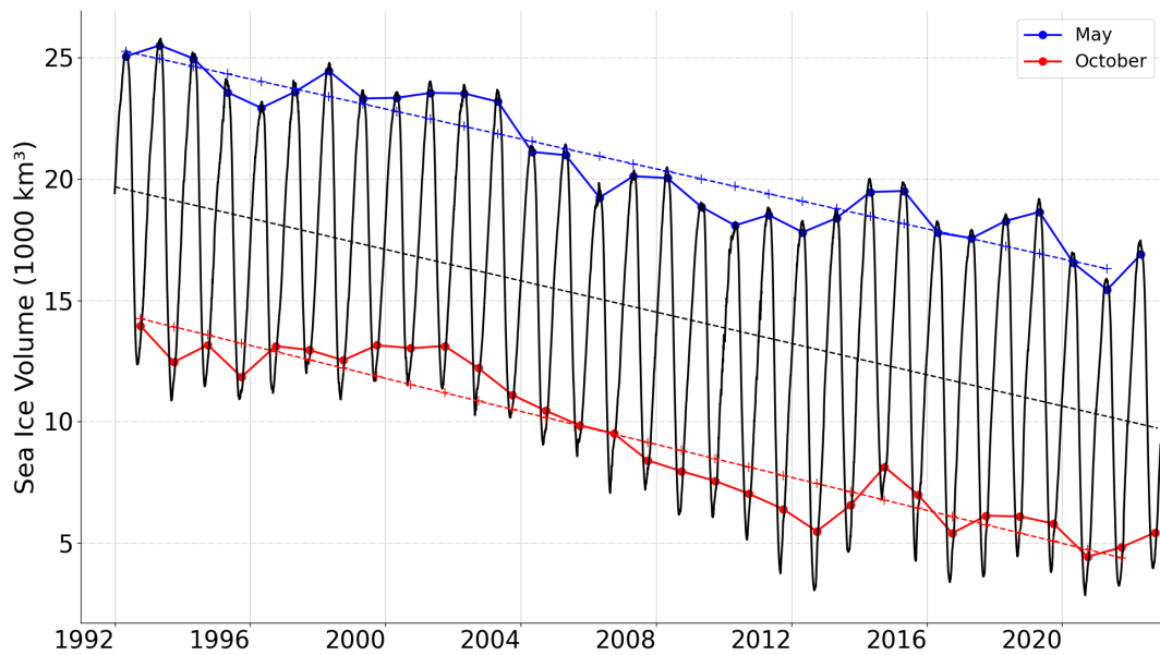
Figure B1. Total sea ice volume (1000 km 3 ) for the entire Arctic domain from 1992 to 2022. The monthly average in May (October) is indicated in blue (red). Trends are depicted for the entire period in dotted lines. It should be noted that the TOPAZ domain excludes the Pacific Seas south of the Bering Strait.
