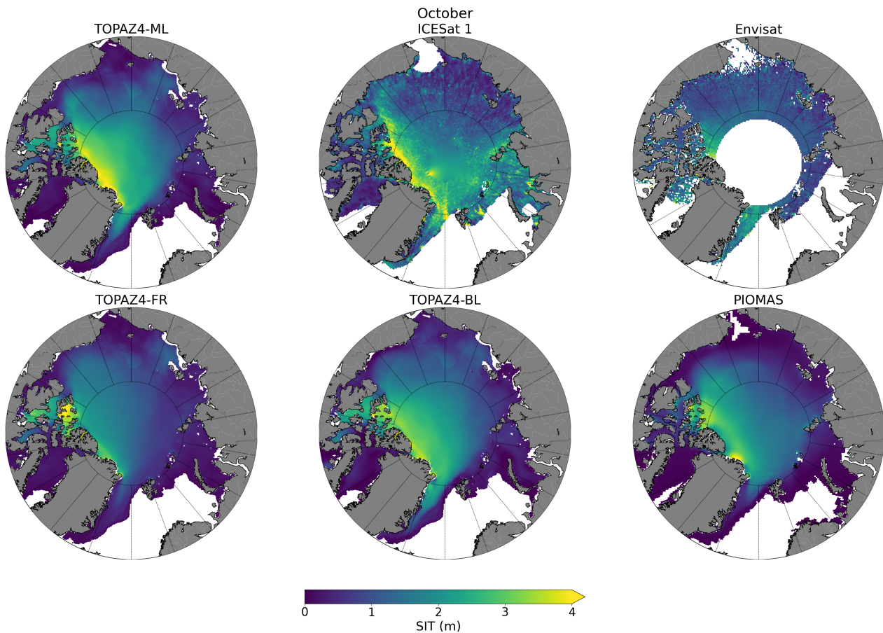
Figure 8. Sea ice thickness (meters) for TOPAZ4-ML, ICESat-1, Envisat, TOPAZ4-FR, TOPAZ4-BL and PIOMAS averaged over October 2003-2007. ICESat-1 observation period varies, extending into November depending on the year.
