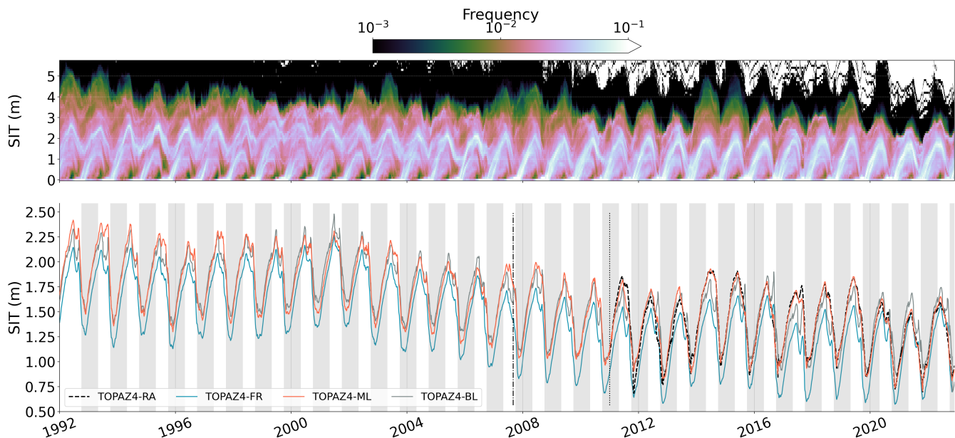
Figure 10. Top) Distribution of daily TOPAZ4-ML SIT (m) from 1992 to 2022. Bins of 0.1m are used and the color bar is a log scale. Bottom) Daily SIT (m) averaged over the Arctic for SIC>15% for the same period. The ML algorithm has been retrained including 2011-2013, as indicated by the vertical line in 2011. The dot-dashed vertical black line marks September 2007. The freezing periods from October to April are highlighted with a grey background.
