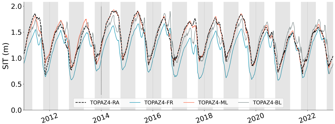
Figure 6. Daily SIT (m) averaged over the Arctic for SIC>15%. SIT for TOPAZ4-RA (considered as our truth), TOPAZ4-FR, TOPAZ4-ML, and TOPAZ4-BL are shown. A vertical line in 2014 separates the test (2011-2013) from the training sets (2014-2022). The freezing periods from October to April are highlighted with a grey background.
