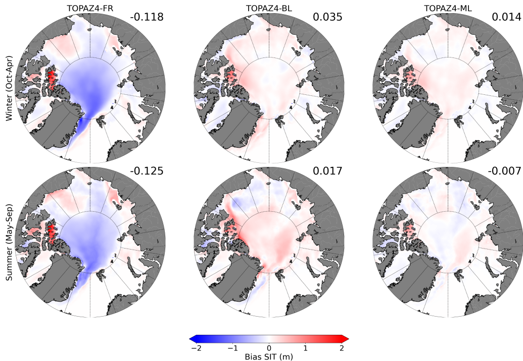
Figure 4. Seasonal bias of SIT (m) averaged over the test period (2011-2013), between left column ) TOPAZ4-FR and TOPAZ4-RA, and middle column ) TOPAZ-BL and TOPAZ4-RA, and right column ) TOPAZ4-ML and TOPAZ4-RA. The blue colour indicates that the TOPAZ4 reanalysis SIT is thicker. The freezing period ( top row ) extends from October to April, while the melting season ( bottom row ) spans from May to September.
