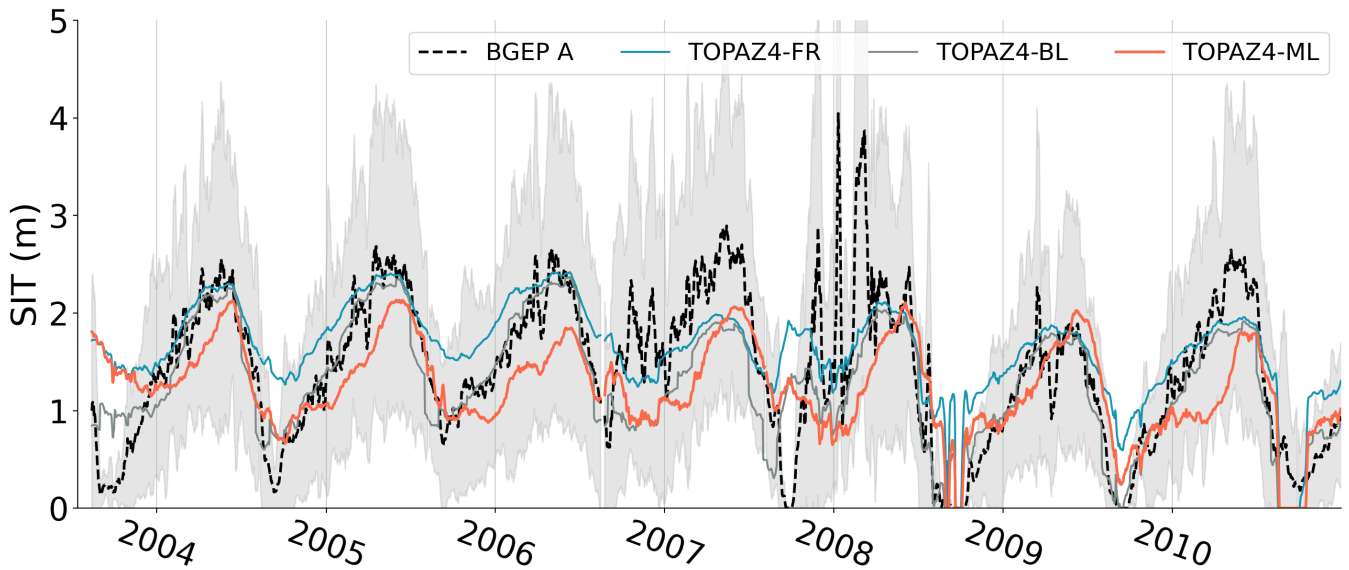
Figure 7. Daily SIT (m) for buoy BGEPA, TOPAZ freerun, baseline, and ML-adjusted. The standard deviation of SIT for ULS BGEPA is displayed in grey.
