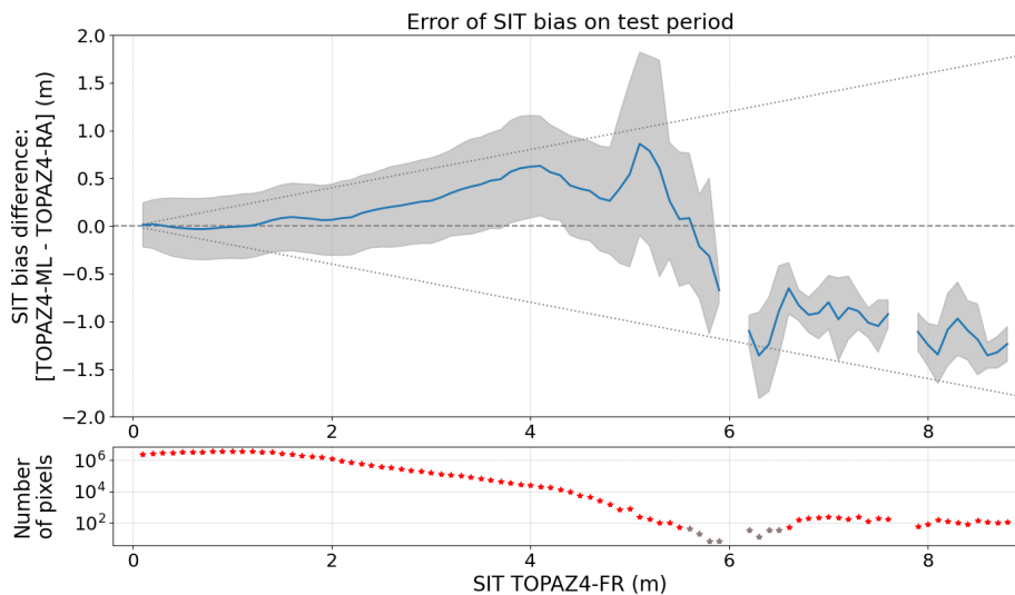
Figure C1. Top) Difference of bias correction between the ML prediction and the true bias correction as a function of the sea ice thickness from TOPAZ4-FR over the test period (2011-2013). The true bias correction is obtained from TOPAZ4-RA - TOPAZ4-FR. Bins of 10 cm are used to average the differences (blue) and their standard deviation (grey). The two oblique lines represent 20% of sea ice thickness for each bin. Positive values indicate that the ML algorithm predicts an excessively high adjustment of sea ice thickness compared to the correction applied by the CS2SMOS data assimilation in TOPAZ4. Bottom) Number of pixels collected in each bin as a function of sea ice thickness estimated by TOPAZ4-FR. Grey stars indicate bins with less than 50 pixels.
