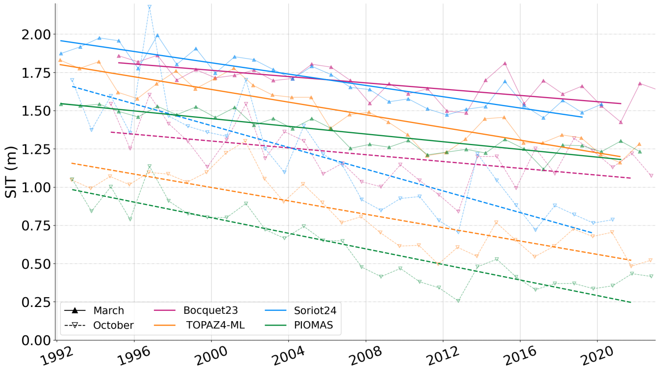
Figure 9. Monthly mean sea ice thickness over the Arctic (latitudes <81.5^\circ N) for March and October from 1992 to 2022. The displayed datasets include TOPAZ4-ML (this study), PIOMAS, Bocquet et al. (2023), and Soriot et al. (2024). Trends are shown for the entire time period.
