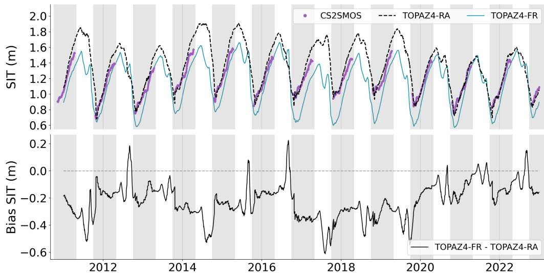
Figure 3. Top) Daily sea ice thickness (m) averaged over the Arctic within the ice edge. TOPAZ4-RA, TOPAZ4-FR, and the CS2SMOS merged-satellites product are displayed. Bottom) Bias of sea ice thickness (m) computed as follows: TOPAZ4-FR - TOPAZ4-RA. The freezing periods from October to April are highlighted with a grey background.
