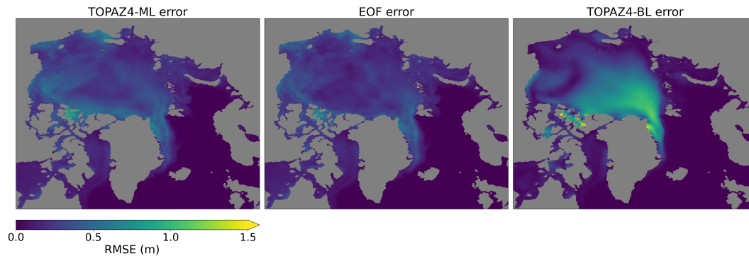
Figure 5. RMSE of SIT bias (m) over the test period (2011-2013) of left ) ML-adjusted error, middle ) EOF error, right ) baseline error against the SIT bias between TOPAZ4-FR and TOPAZ4-RA.
