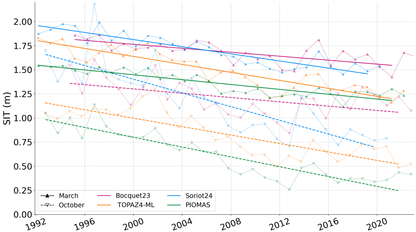
Figure 9. Monthly mean sea ice thickness over the Arctic (latitudes <81.5^{\circ} N) for March and October from 1992 to 2022. The displayed datasets include TOPAZ4-ML (this study), PIOMAS, Bocquet et al. (2023), and Soriot et al. (2024). Trends are shown for the entire time period.
