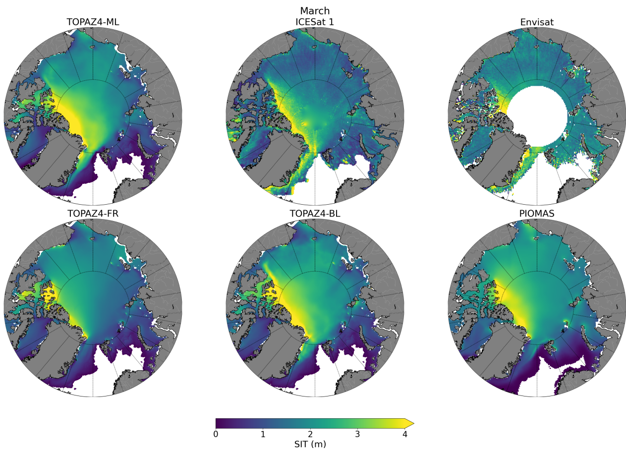
Figure S3. Sea ice thickness (meters) for TOPAZ4-ML, ICESat-1, Envisat, TOPAZ4-FR, and TOPAZ4-BL and PIOMAS averaged over March 2003-2007. ICESat-1 observation period varies, including days in February or in April depending on the year.
