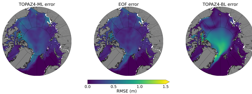
Figure 5. RMSE of SIT bias (m) over the test period of a) (2011-2013) of left ) ML-adjusted error, b) middle ) EOF error, c) right ) baseline error against the SIT bias between TOPAZ4-FR and TOPAZ4-RA.
