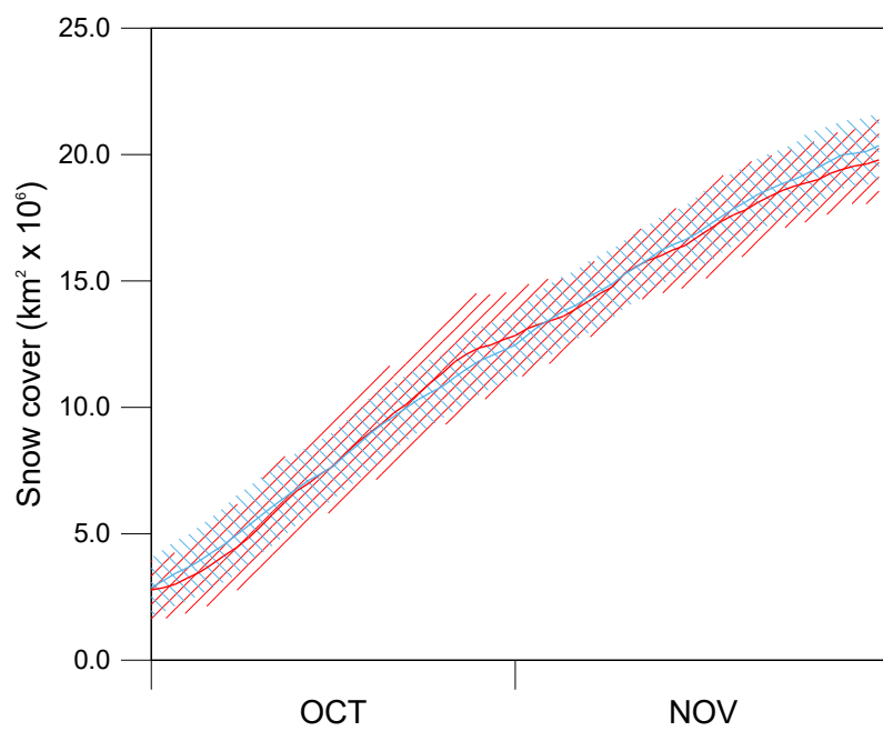
Figure S2. Comparison of Eurasian snow cover between ERA5 (red) and offset 20CRv3 (blue) for 2003-2015. Shading represents one standard deviation either side of the mean.
