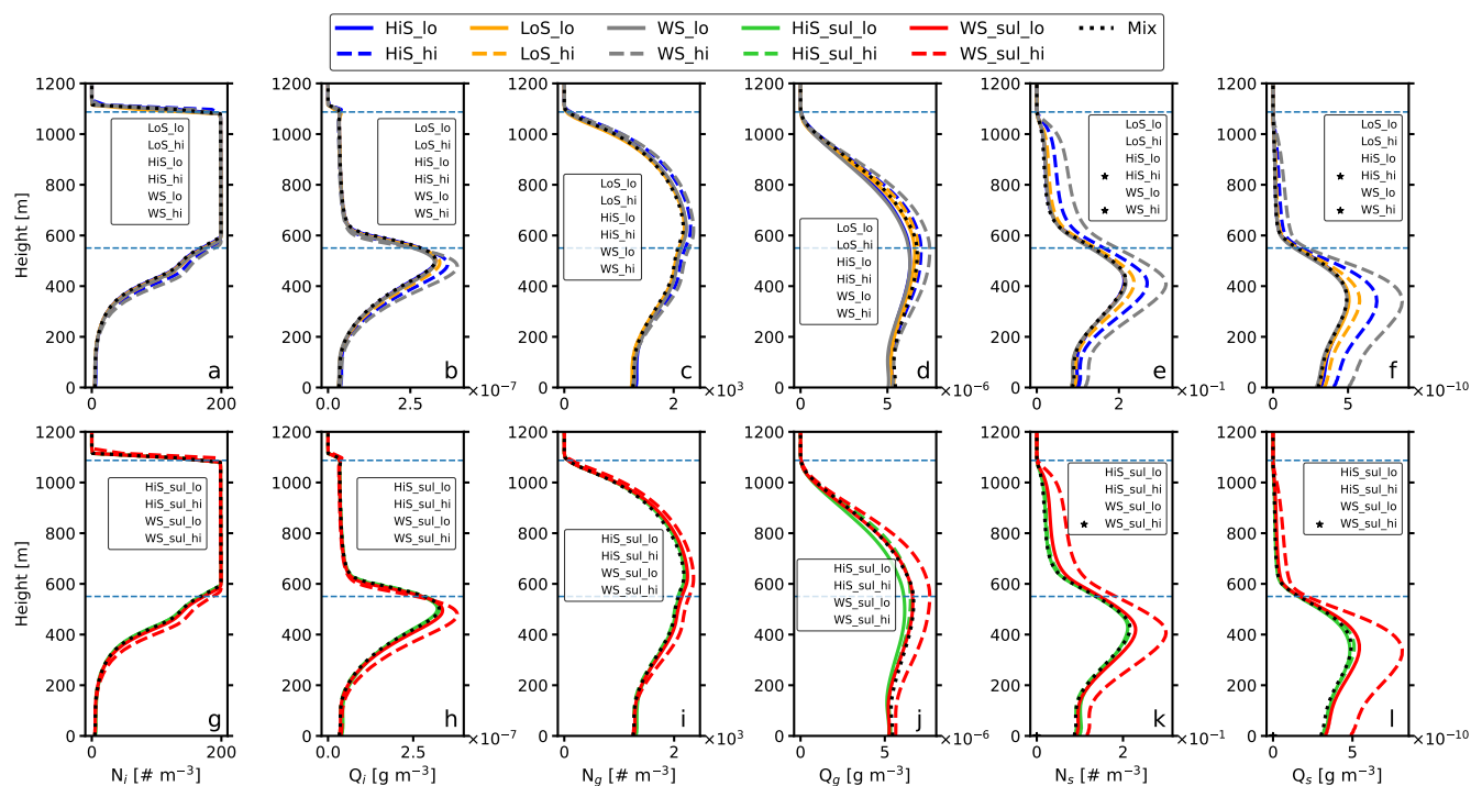
Figure C1. Vertical profiles of horizontally averaged (a and g) N_i , (b and h) Q_i , (c and i) N_g , (d and j) Q_g , (e and k) N_s and (f and l) Q_s averaged over the last four simulation hours. The light blue, dashed line represents the average cloud bottom and top height calculated for the reference case (Mix). HiS, LoS, and WS represent ship aerosol from measurements of high and low sulfur content fuels and wet scrubbing respectively (Santos et al., 2022, 2023). The HiS_sul and WS_sul cases represent sulfate particle modes of high FSC fuel combustion and exhaust gas wet scrubbing from Santos et al. (2024). The label additions _lo and _hi signify the ship aerosol concentrations used in the individual model runs. Significant differences between ship exhaust cases and Mix were assessed using two-sided t tests at a confidence level of 95 %. Model runs with significant differences are marked with star icons in inset legends.
