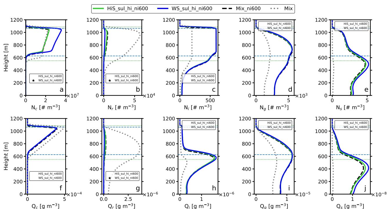
Figure 7. Vertical profiles of horizontally averaged (a) N_c , (b) N_r , (c) N_i , (d) N_g , (e) N_s , (f) Q_c , (g) Q_r , (h) Q_i , (i) Q_g and (j) Q_s averaged over the last four simulation hours for Mix_ni600, HiS_sul_hi_ni600, WS_sul_hi_ni600 and Mix. The light blue, dashed line represents the average cloud bottom and top height calculated for Mix_ni600 (green, dotted line for Mix respectively). The HiS_sul and WS_sul cases represent sulfate particle modes of high FSC fuel combustion and exhaust gas wet scrubbing. Significant differences between ship exhaust cases and Mix_ni600 were assessed using two-sided t tests at a confidence level of 95%. Model runs with significant differences are marked with star icons in inset legends.
