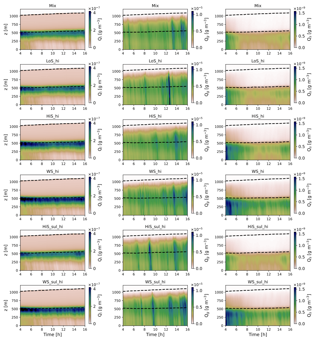
Figure B2. Temporal evolution of horizontally averaged mixing ratios of ice crystals ( Q_i ), graupel ( Q_g ) and snow ( Q_s ) simulated for the reference case (Mix) and the high ship aerosol concentration cases LoS_hi, HiS_hi, WS_hi, HiS_sul_hi and WS_sul_hi. The black dashed lines represent case-specific, horizontally averaged cloud bottom and cloud top heights. The spin-up period (0 to 4 h) is removed from all figures.
