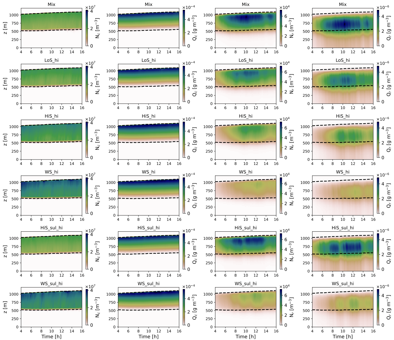
Figure 3. Temporal evolution of horizontal domain averaged cloud droplet number concentrations ( N_c ; [ N_c ] = \text{m}^{-3} ), cloud droplet mixing ratios ( Q_c ; [ Q_c ] = \text{g m}^{-3} ), raindrop number concentrations ( N_r ) and raindrop mixing ratios ( Q_r ) simulated for the reference case (Mix) and the high ship aerosol concentration cases LoS_hi, HiS_hi, WS_hi, HiS_sul_hi and WS_sul_hi. The black dashed lines represent case-specific, horizontally averaged cloud bottom and cloud top heights. The spin-up period (0 to 4 h) is removed from all figures.
