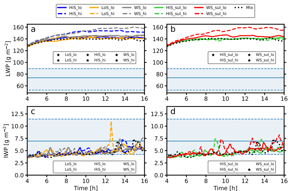
Figure 2. Time evolution of the simulated domain-averaged (a and b) liquid water path (LWP) and (c and d) ice water path (IWP). Mix refers to the reference case with background aerosol only. HiS, LoS, and WS represent ship aerosol from measurements of high and low sulfur content fuels and wet scrubbing respectively (Santos et al., 2022, 2023). The HiS_sul and WS_sul cases represent sulfate particle modes of high FSC fuel combustion and exhaust gas wet scrubbing from Santos et al. (2024). The label additions _lo and _hi signify the ship aerosol concentrations used in the individual model runs. Significant differences between ship exhaust cases and Mix were assessed using two-sided t tests at a confidence level of 95%. Model runs with significant differences are marked with star icons in inset legends. For the statistical tests the last 4 simulation hours were used. The blue shaded area refers to the retrieved LWP and IWP from microwave radiometer measurements (median over the observation period; the corresponding dashed lines are the 25th/75th percentiles) during the ASCOS campaign (Tjernström et al., 2012, 2014) which were used to initialize the model. The first four hours are considered a spin-up period of the model and are removed from the figures.
