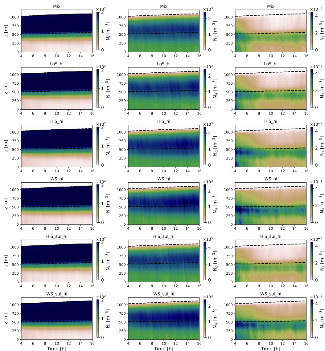
Figure B1. Temporal evolution of horizontally averaged number concentrations of ice crystals ( N_i ), graupel ( N_g ) and snow ( N_s ) simulated for the reference case (Mix) and the high ship aerosol concentration cases LoS_hi, HiS_hi, WS_hi, HiS_sul_hi and WS_sul_hi. The black dashed lines represent case-specific, horizontally averaged cloud bottom and cloud top heights. The spin-up period (0 to 4 h) is removed from all figures.
