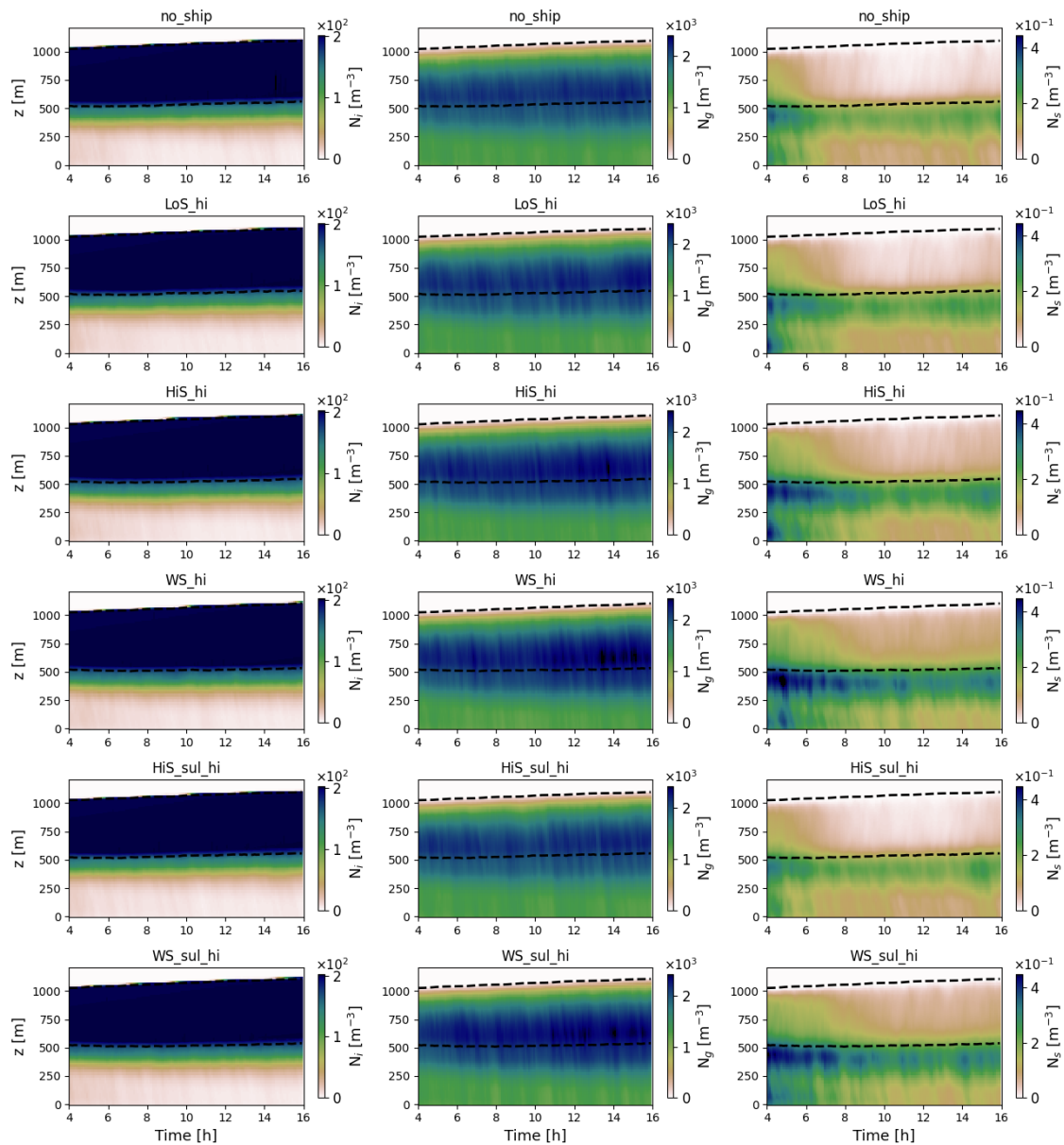
Figure B1. Temporal evolution of horizontally averaged number concentrations of ice crystals ( N_i ), graupel ( N_g ) and snow ( N_s ) simulated for the reference case (no_ship) and the high ship aerosol concentration cases LoS_hi, HiS_hi, WS_hi, HiS_sul_hi and WS_sul_hi. The black dashed lines represent case-specific, horizontally averaged cloud bottom and cloud top heights. The spin-up period (0 to 4 h) is removed from all figures.
