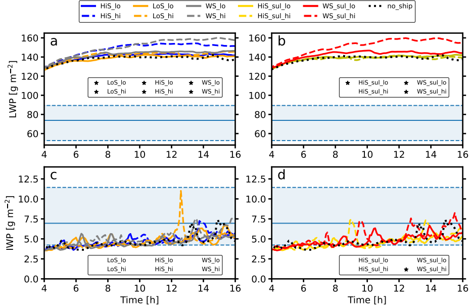
Figure 2. Time evolution of the simulated domain-averaged (a and b) liquid water path (LWP) and (c and d) ice water path (IWP). no_ship refers to the reference case with background aerosol only. HiS, LoS, and WS represent ship aerosol from measurements of high and low sulfur content fuels and wet scrubbing respectively (Santos et al., 2022, 2023). The HiS_sul and WS_sul cases represent sulfate particle modes of high FSC fuel combustion and exhaust gas wet scrubbing from Santos et al. (2024b). The label additions _lo and _hi signify the ship aerosol concentrations used in the individual model runs. Significant differences between ship exhaust cases and no_ship were assessed using two-sided t tests at a confidence level of 95%. Model runs with significant differences are marked with star icons in inset legends. For the statistical tests the last 4 simulation hours were used. The blue shaded area refers to the retrieved LWP and IWP from microwave radiometer measurements (median over the observation period; the corresponding dashed lines are the 25th/75th percentiles) during the ASCOS campaign (Tjernström et al., 2012, 2014) which were used to initialize the model. The first four hours are considered a spin-up period of the model and are removed from the figures.
