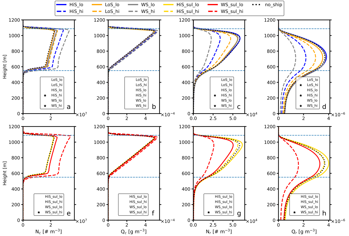
Figure 4. Vertical profiles of horizontally averaged (a and e) N_c , (b and f) Q_c , (c and g) N_r and (d and h) Q_r averaged over the last four simulation hours. The light blue, dashed line represents the average cloud bottom and top height calculated for the reference case (no_ship). HiS, LoS, and WS represent ship aerosol from measurements of high and low sulfur content fuels and wet scrubbing respectively (Santos et al., 2022, 2023). The HiS_sul and WS_sul cases represent sulfate particle modes of high FSC fuel combustion and exhaust gas wet scrubbing from Santos et al. (2024b). The label additions _lo and _hi signify the ship aerosol concentrations used in the individual model runs. Significant differences between ship exhaust cases and no_ship were assessed using two-sided t tests at a confidence level of 95%. Model runs with significant differences are marked with star icons in inset legends.
