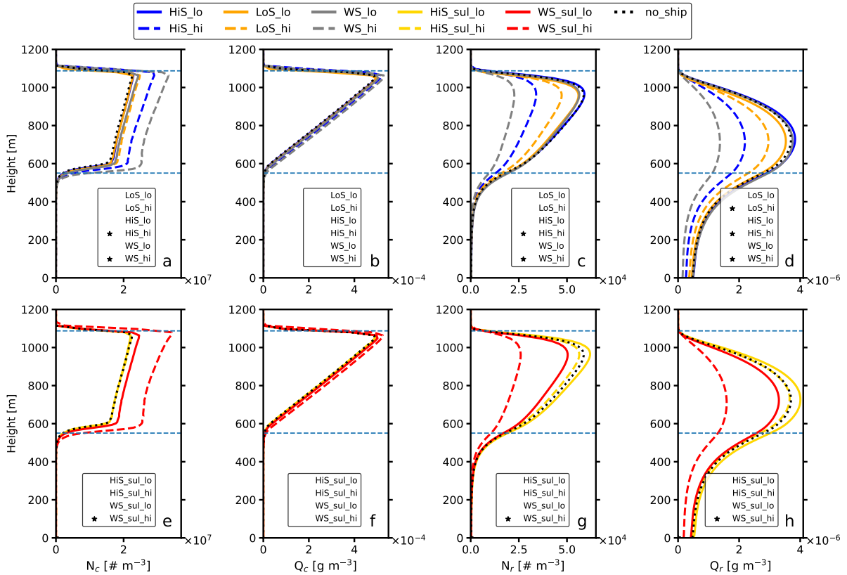
Figure 4. Vertical profiles of horizontally averaged (a and e) N_c , (b and f) Q_c , (c and g) N_r , and (d and h) Q_r , averaged over the last four simulation hours. The light blue, dashed line represents the average cloud bottom and top height calculated for the reference case ( Mix-no_ship ). HiS, LoS, and WS represent ship aerosol from measurements of high and low sulfur content fuels and wet scrubbing respectively (Santos et al., 2022, 2023). The HiS_sul and WS_sul cases represent sulfate particle modes of high FSC fuel combustion and exhaust gas wet scrubbing from Santos et al. (2024b). The label additions _lo and _hi signify the ship aerosol concentrations used in the individual model runs. Significant differences between ship exhaust cases and Mix-no_ship were assessed using two-sided t tests at a confidence level of 95%. Model runs with significant differences are marked with star icons in inset legends.
