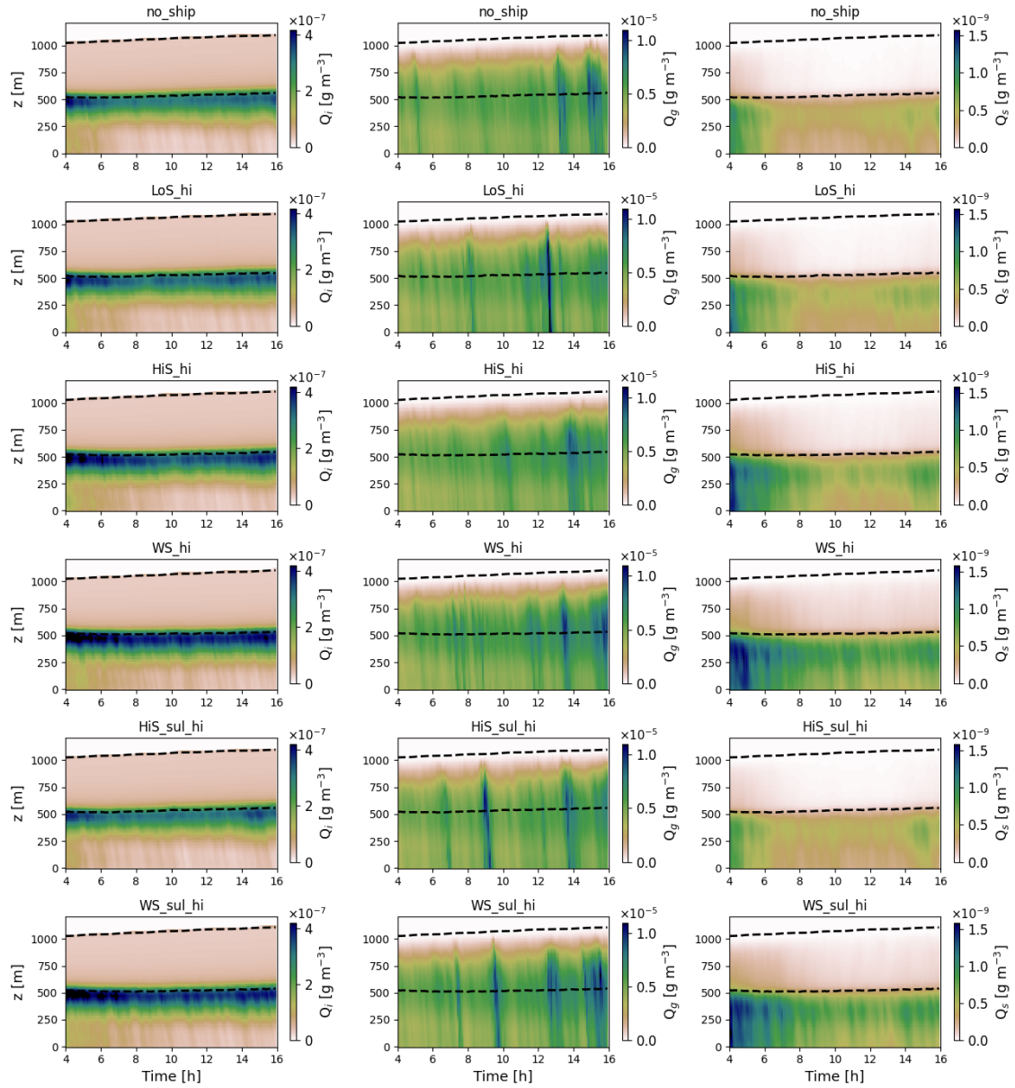
Figure B2. Temporal evolution of horizontally averaged mixing ratios of ice crystals ( Q_i ), graupel ( Q_g ) and snow ( Q_s ) simulated for the reference case ( Mixno_ship ) and the high ship aerosol concentration cases LoS_hi, HiS_hi, WS_hi, HiS_sul_hi and WS_sul_hi. The black dashed lines represent case-specific, horizontally averaged cloud bottom and cloud top heights. The spin-up period (0 to 4 h) is removed from all figures.
