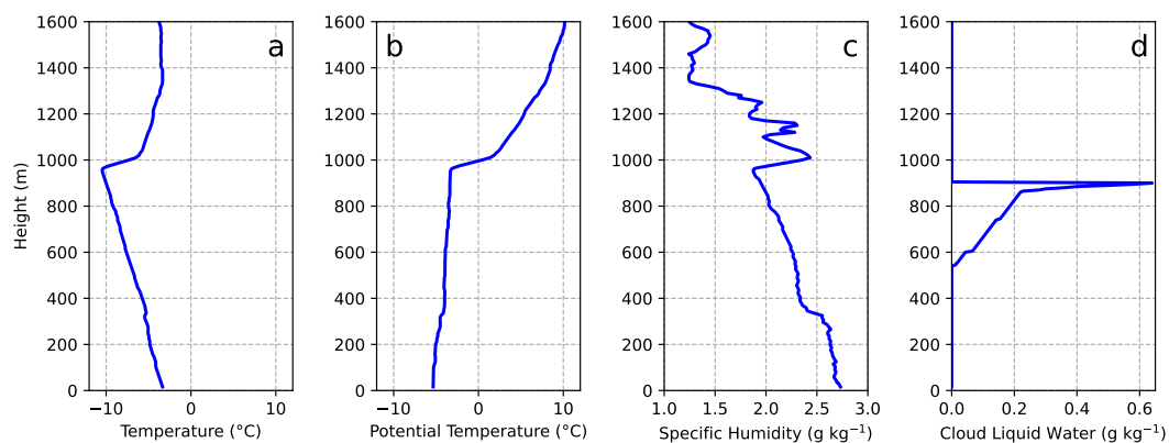
Figure A1. Radiosonde observations of (a) temperature, (b) potential temperature, (c) specific humidity and (d) derived cloud liquid water based on radiometer measurements performed on August 31st 2008 during the ASCOS campaign (Tjernström et al., 2012, 2014). The data was used to initialize MIMICA in this study.
