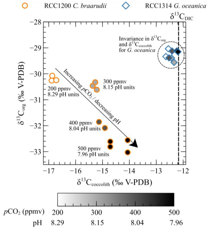
405 Figure 8: Scatter plot showing \delta^{13}\text{C}_{\text{org}} versus \delta^{13}\text{C}_{\text{coccolith}} values with changes in p\text{CO}_2 and pH (circles: Coccolithus braarudii , RCC 1200; diamonds: Gephyrocapsa oceanica , RCC 1314). Grey levels correspond to growth conditions (white: 200 ppmv/8.29 pH units, light grey: 300 ppmv/8.15 pH units, dark grey: 400 ppmv/8.04 pH units, black: 500 ppmv/7.96 pH units).
