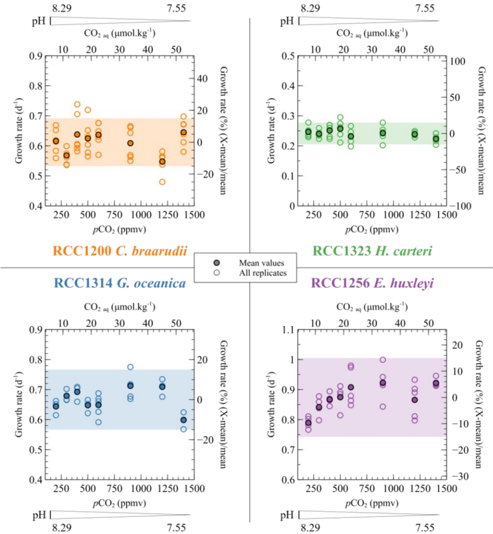
230 Figure 2: Specific growth rate ( \mu ) of the four cultured strains with respect to CO 2 level and pH of the culture media. The empty dots show all the replicate data and the filled dots denote the mean growth rates. Growth rates are given in \text{d}^{-1} (left axis) and as a relative deviation of the mean growth rate of each strain (right axis). The coloured bands correspond to the range of \pm 15\% of variation from the mean growth rate. More than 85% of the data are comprised within this range.
