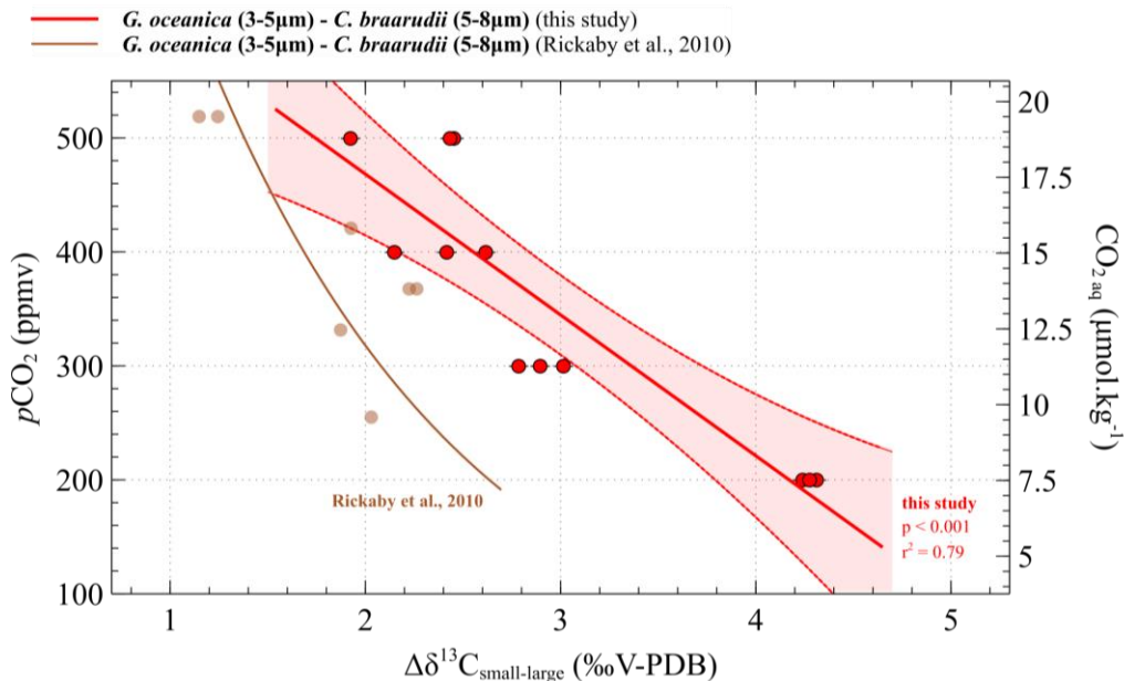
Figure 9: Calibration between \text{CO}_2 and \Delta\delta^{13}\text{C}_{\text{small-large}} obtained from culture experiments. The results of our study are shown in red (replicate data as dots, the linear regression made between 200 and 500 ppmv corresponds to the solid line and the confidence interval is shown with dotted lines). The brown curve is the equation recalculated from Rickaby et al. (2010) dataset. The relation encompassing the 200-1400 ppmv spectrum is shown in Figure A1.
