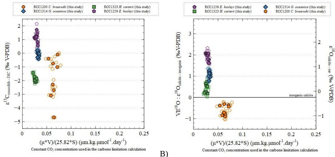
535 Figure A4: Carbon (A) and oxygen (B) isotopic effect with changes in the carbon limitation calculated as for Figure A3 with the difference that the CO 2 concentration is a constant (25.82 μmol.kg -1 , mean CO 2 concentration of the medium conditions in this study).
