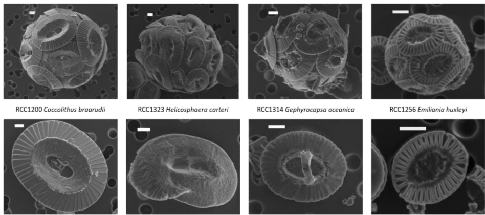
105 Figure 1: Scanning electron microscope (SEM) images of the four studied strains. Top images show the coccoliths-coccospheres and bottom images show the coccospheres-coccoliths. The scale bars represent 1 μm.
