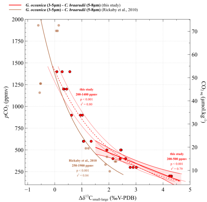
Figure A1: Calibration between CO_2 concentrations and \Delta\delta^{13}C_{\text{small-large}} obtained from culture experiments at low and high CO_2 levels. The results of our study are shown in red. Replicate data are illustrated with red dots. The linear regression made between 200 and 500 ppmv corresponds to the solid line and the confidence interval is shown with dotted lines. The dotted line shows the logarithmic regression made for the data on the whole interval (200 to 500 ppmv). The brown curve is the equation recalculated from Rickaby et al. (2010) dataset.
