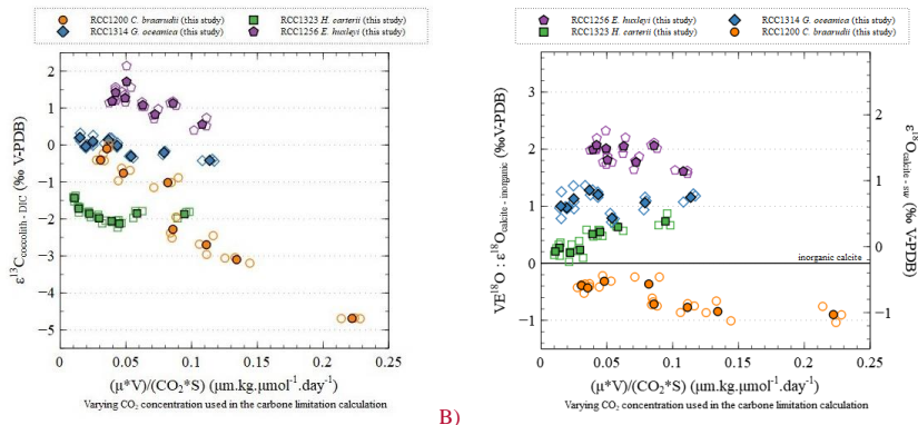
Figure A3: Carbon (A) and oxygen (B) isotopic effect with changes in the carbon limitation. Carbon limitation is calculated as the product of growth rate ( \mu , in \text{day}^{-1} ) and coccosphere volume ( V , in \mu\text{m}^3 ) divided by the product of CO 2 concentration (CO 2 , in \mu\text{mol.kg}^{-1} ) and coccosphere surface ( S , in \mu\text{m}^2 ), according to Bidigare et al., 1997.
