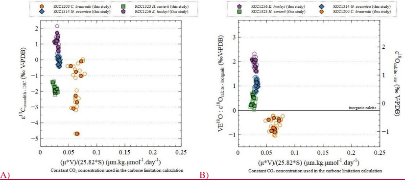
Figure A4: Carbon (A) and oxygen (B) isotopic effect with changes in the carbon limitation calculated as for Figure A3 with the difference that the \text{CO}_2 concentration is a constant ( 25.82 \mu\text{mol.kg}^{-1} , mean \text{CO}_2 concentration of the medium conditions in this study).
