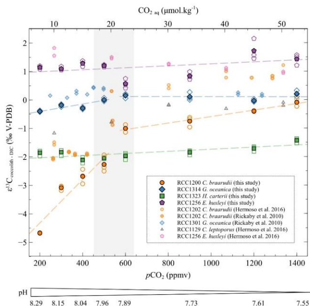
Figure 5: Evolution of the carbon isotopic ratios of the four studied strains with increasing CO 2 concentration and decreasing pH. The data are represented as the \delta^{13}\text{C} difference-fractionation between coccoliths and DIC. The empty points are all the replicate data and the filled points are the means (circles: Coccolithus braarudii , RCC 1200; diamonds: Gephyrocapsa oceanica , RCC 1314; squares: Helicosphaera carteri ; pentagons: Emiliania huxleyi ). The grey band represents the carbonate chemistry condition where a shift in the carbon and oxygen isotope ratio occurs (between 500 and 600 ppmv). The pH indicated below only refers to the pH of the cultures of this study. The sources of previously reported data (smaller symbols) are inset.
