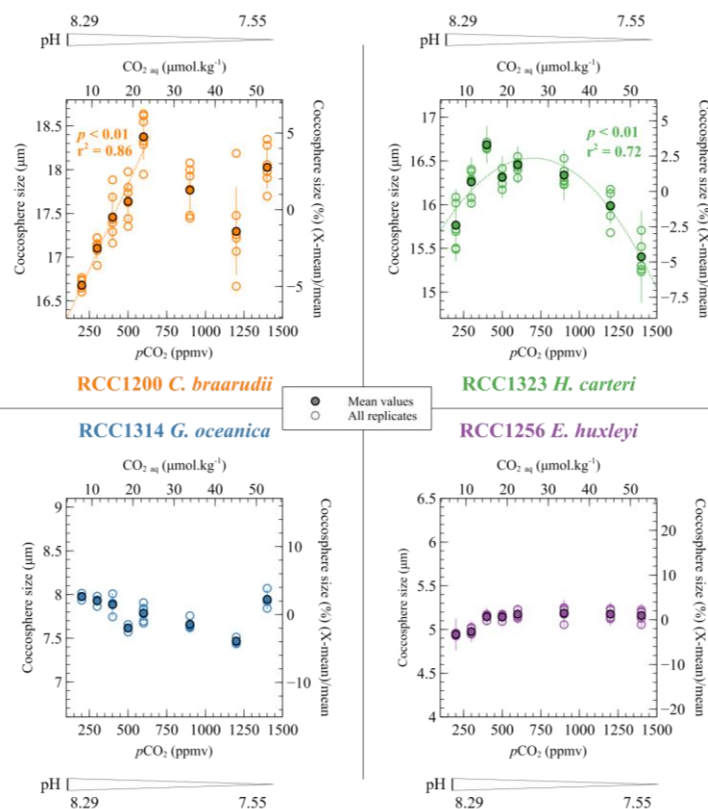
Figure 3: Evolution of the coccosphere sizes of the four cultured strains as a function of the \text{CO}_2 and pH culture conditions. The coccosphere sizes are given as the mean diameter of the coccospheres. They are given in \mu\text{m} (left axis) and as a percent relative to the mean coccosphere size of each strain (right axis). The empty points show the replicate data and the filled points show the mean coccosphere sizes.
