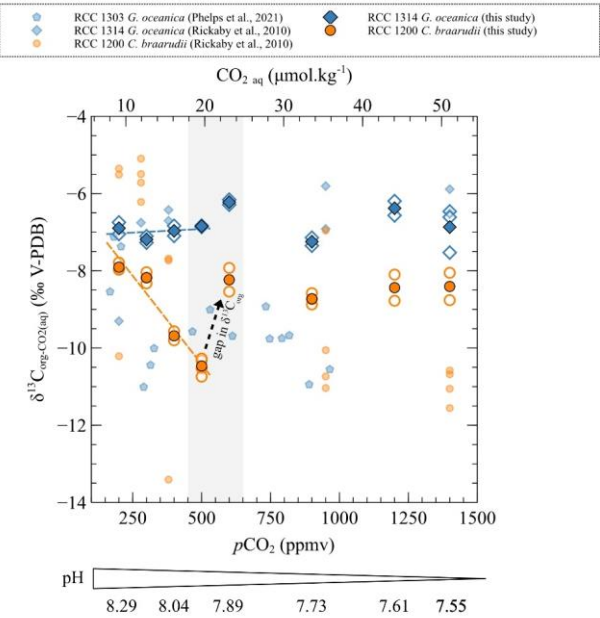
345 Figure 7: Carbon isotopic ratios of organic matter compared to \delta^{13}\text{C}_{\text{CO}_2(\text{aq})} of the strains studied with changes in CO 2 level and pH. The empty points are all the replicate data and the filled points are the means. The grey band represents the carbonate chemistry condition where a shift in the carbon and oxygen isotope ratio occurs. The sources of previously reported data (smaller symbols) are inset.
