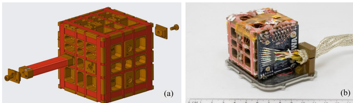
Figure 1: (a) The Tesseract magnetometer design secures six miniature low noise racetrack cores within a symmetric block of 30% glass-filled Torlon engineering plastic. These racetrack cores, developed by Miles et al., 2022, are wrapped in a quasi-toroidal drive winding to modulate the permeability of the core and then covered in a solenoidal sense winding to sense the modulated signal. The Tesseract's feedback coils are wound on the same glass-filled Torlon base for structural stability. These feedback coils (red) are arranged in a three axis four-loop Merritt coil which creates a large region of magnetic homogeneity inside the sensor. (b) A photograph of the as-built Tesseract sensor that was flown on the ACES-II-Low sounding rocket.
