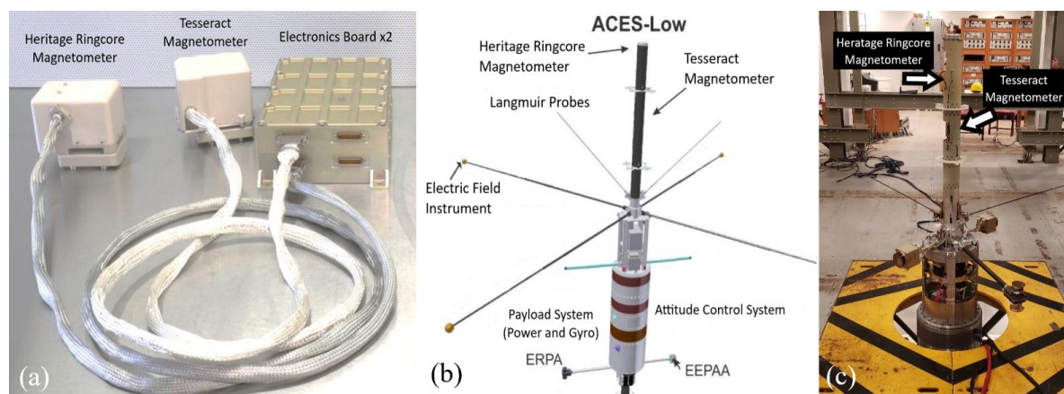
135 Figure 3: (a) A photograph of the magnetometer instruments which flew on the ACES-II Low. The electronics boards for each sensor are stacked on top of one another. (b) A diagram of the ACES-II-Low science instrument payload. The Tesseract and Ringcore sensors 140 are mounted in the rocket mast. The Tesseract is mounted inboard and the Ringcore is mounted outboard. (c) The Tesseract magnetometer and Ringcore magnetometer under test at the Wallops calibration facility while mounted on the rocket.
