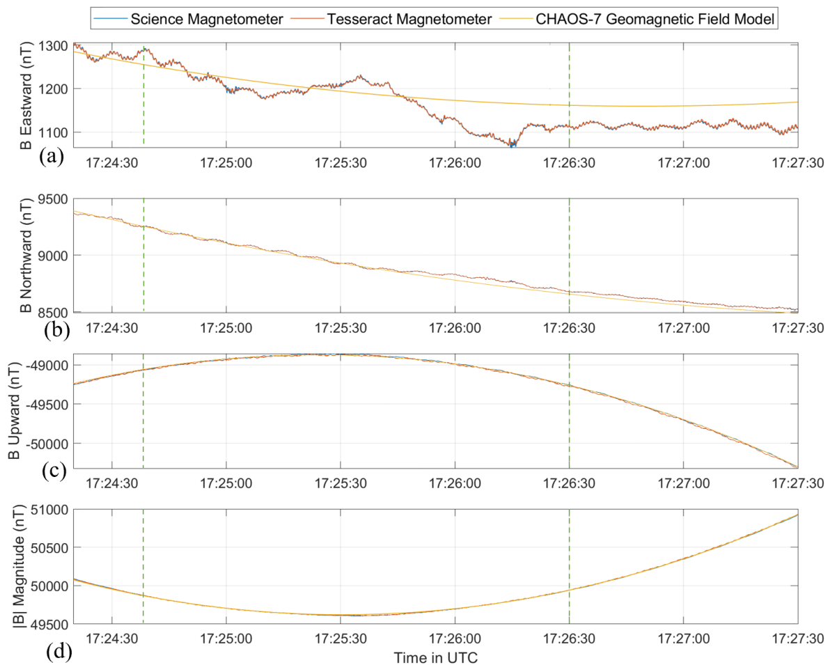
260 Figure 6: During a quiet segment of data, between 17:24:00 and 17:24:30, the Ringcore and Tesseract data was calibrated using the 265 calibration values obtained during preflight testing. The magnetic field measured by the Tesseract magnetometer is plotted over time in red, and the measured field by the ring core is plotted in blue for the Eastward (a), Northward (b) and Upward (c) directions. The scalar magnetic field is plotted in (d). The magnetic field predicted by the CHAOS 7 geomagnetic field model was evaluated at the rocket's location over the course of the flight and is plotted in yellow. The region where we expect to observe auroral activity based on the All- sky image is bounded by green dotted lines.
