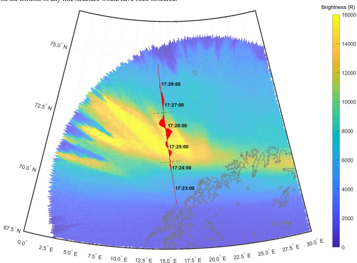
Figure 7: An All-Sky image taken in Skiboten, Norway at 17:25:30 is projected onto its approximate location and is plotted alongside the trajectory of the ACES-II lowflyer as measured by the rocket GPS. The eastward DC magnetic field that Tesseract magnetometer measures over the course of the flight is plotted in red. Around the apogee, from 17:24:40 UTC to 17:26:30 UTC, the ACES-II low flyer passes through at least one an active auroral arc.
