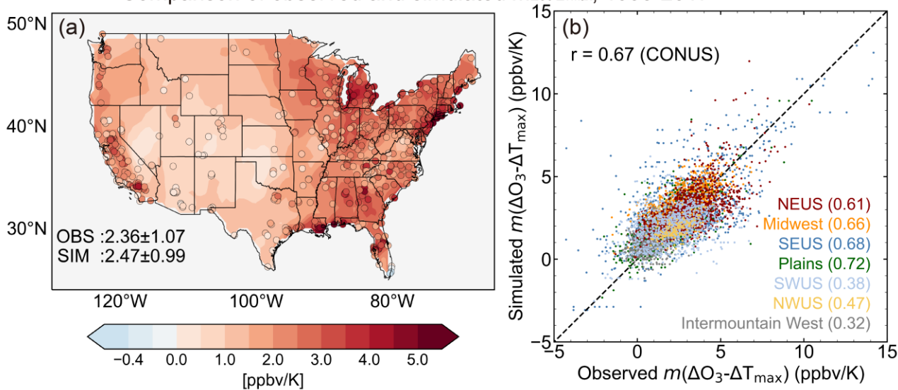
Comparison of observed and simulated m_{\Delta O_3-\Delta T_{max}} , 1995-2017
