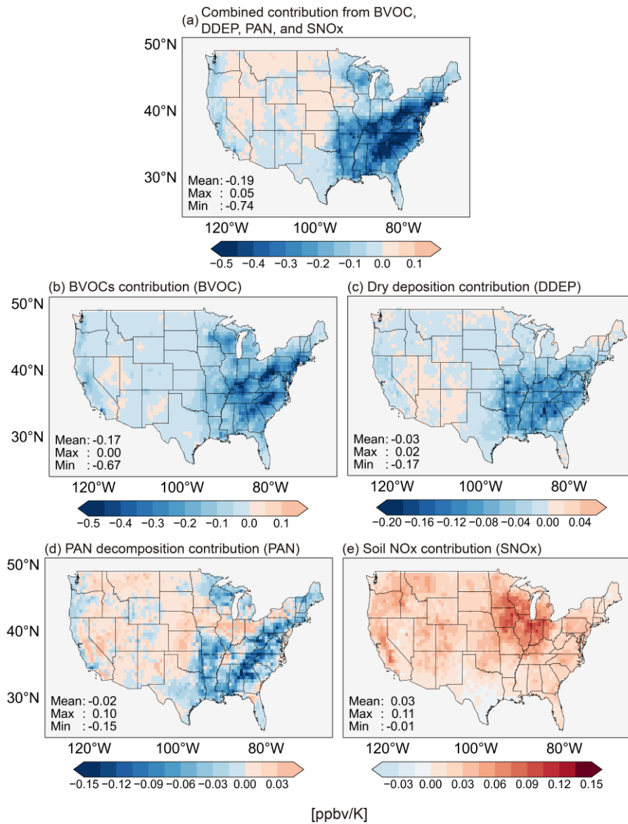
440 Figure 8. The different temperature- indirect direct effects for the decrease in m_{\text{AO3-ATmax}} with anthropogenic \text{NO}_x emission reduction. (a) Combined contribution of the four temperature-dependent mechanisms (BVOCs emissions, dry deposition, PAN decomposition, and soil \text{NO}_x emissions) to m_{\text{AO3-ATmax}} with changes in anthropogenic \text{NO}_x emissions, estimated as the difference of m_{\text{AO3-ATmax}} between BASE and 1995E minus the difference between BASE- FALLF4PATHS and 1995E- FALLF4PATHS (Section 2.4). (b)-(e) Individual contribution of BVOCs emissions, dry deposition, PAN decomposition, and soil \text{NO}_x emissions) to m_{\text{AO3-ATmax}} with changes in anthropogenic \text{NO}_x emissions, respectively. Mean, maximum, and minimum values of the contributions among all CONUS sites are shown inset. Note that the data range of each figure is different. 445
