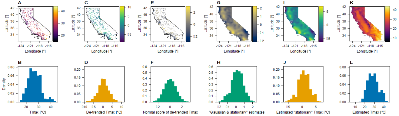
120 Figure 2: Illustration of data processing steps. Each column corresponds to a step in the processing and estimation pipeline. The top row shows point (panels A, C, E) and gridded (panels G, I, K) data values. The bottom row shows histograms of the data at each processing step. Panels A-B show the measured Tmax values. Panels C-D show the Tmax values after spatial trends have been estimated and subtracted. Panels E-F show the detrended Tmax data after the normal score transform has been applied. Panels G-H show gridded estimates produced by OK in the detrended and Gaussian space. Panels I-J show gridded estimates after reverting the normal score transform using quantile information from the distributions in panels C-D. Panels K-L show the final gridded estimates after re-adding spatial trends.
