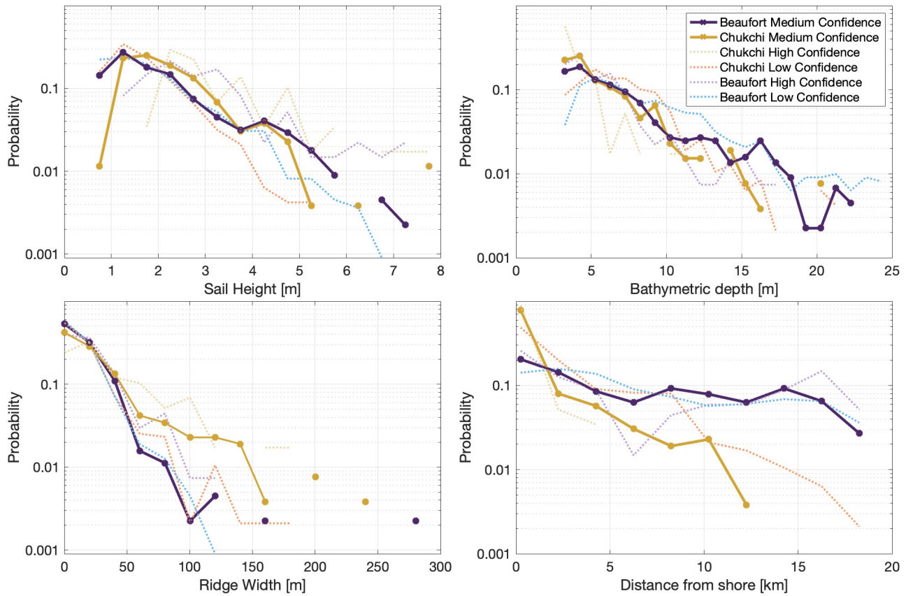
Figure 9. Probability plot for ridge height, depth, width, and distance from shore. The bold yellow (Chukchi) and purple (Beaufort) lines show medium confidence ridges, with the dotted yellow and purple lines showing high confidence ridges and orange and blue indicating low confidence detections.
