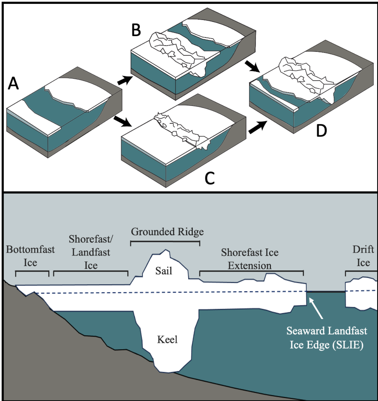
Figure 1. Two mechanisms drive the grounded ridge formation process with (A) the formation of bottom-fast ice attached to shore, (B) a ridge drifts into shallow water and becomes grounded or (C) drifting pack ice colliding to form a deformation ridge, and culminating in (D) the ridge is deep enough to embed in the sea floor. The lower panel shows a cross section of a grounded ice ridge during the winter, not to scale. I is bottomfast ice, II is grounded shorefast ice, III is the grounded ridge, IV is the landfast ice extension, and V is drifting pack ice. The seaward landfast ice edge (SLIE) represents the boundary between shorefast ice and a flaw lead or drifting pack ice.
