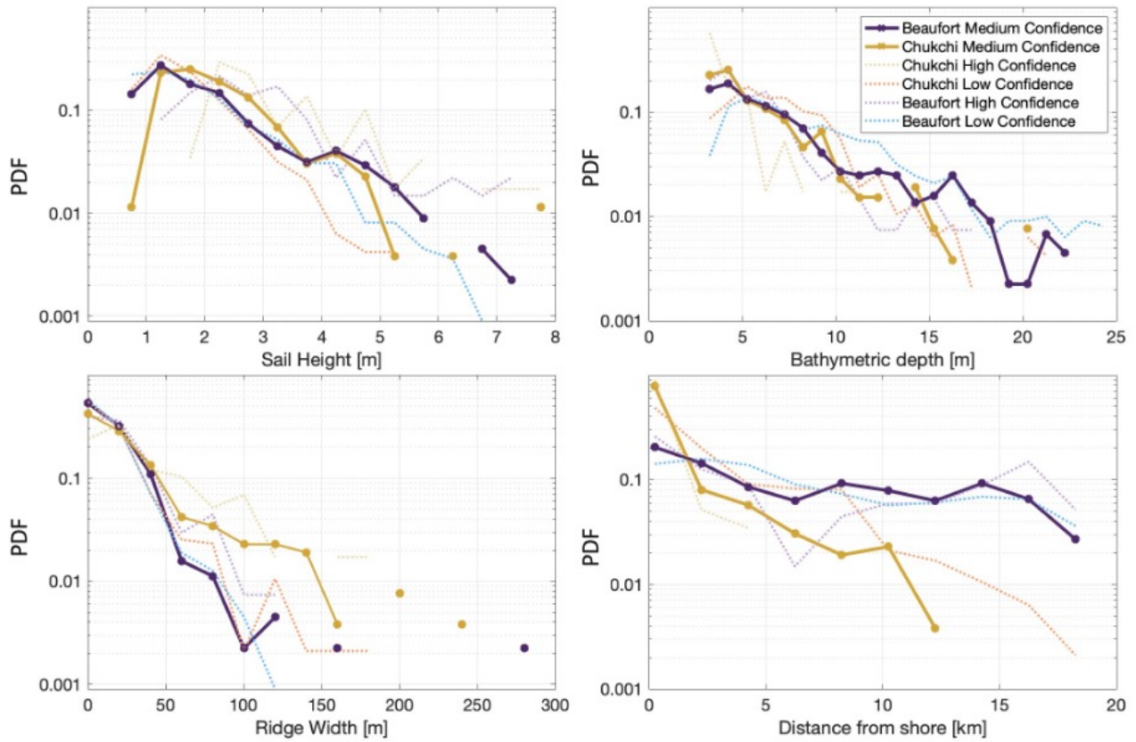
Figure 9. Probability plot density function (PDF) for ridge height, depth, width, and distance from shore. The bold yellow (Chukchi) and purple (Beaufort) lines show medium confidence ridges, with the dotted yellow and purple lines showing high confidence ridges and orange and blue indicating low confidence detections.
