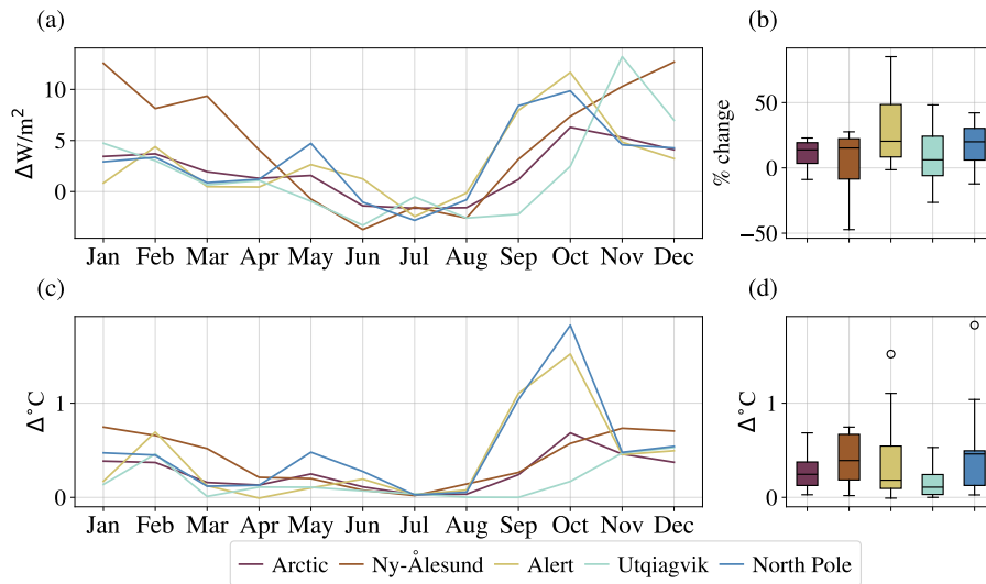
Figure 14. The change in net cloud radiative effect (a-b) and surface air temperature (c-d) between A21 and M92, averaged over the period 2007-04-01 to 2010-03-31. Left: absolute change for each month averaged over selected regions. Right: the distribution of relative change over the months in the same regions.
