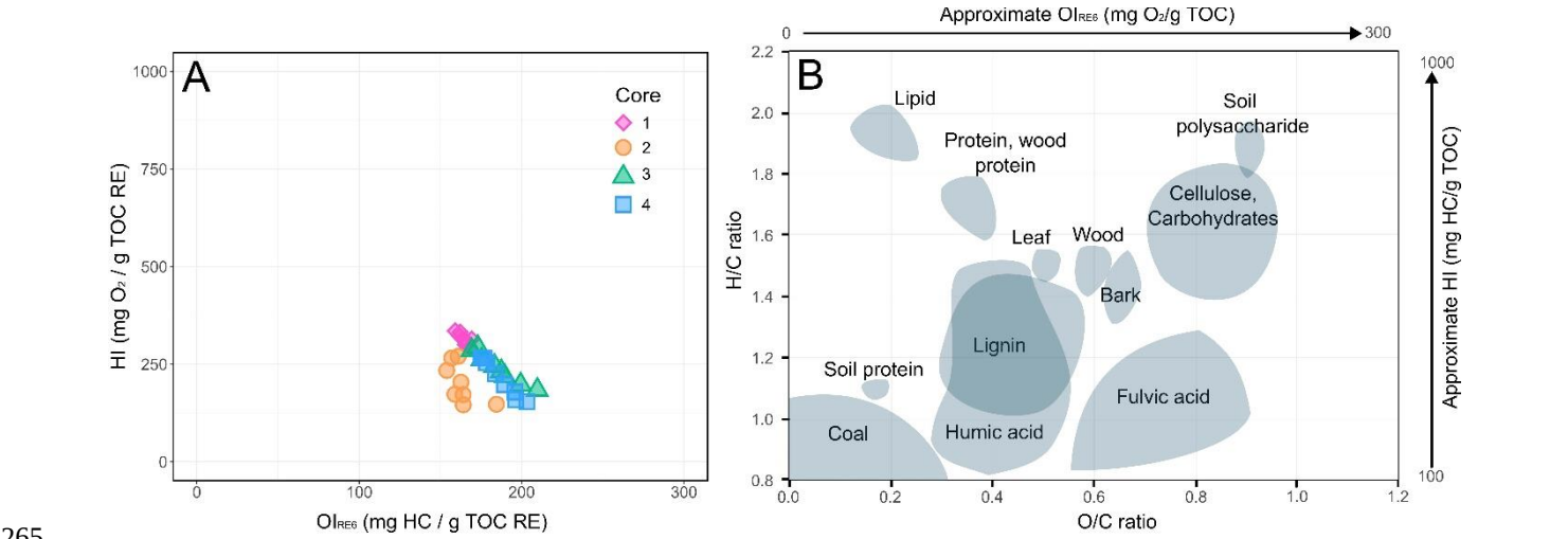
Figure 2: (A) Position of soil samples in the pseudo Van Krevelen diagram (HI vs. OI RE6 ) according to the different soil cores. (B) location of soil molecules and biological compounds in the Van Krevelen diagram (H/C vs. O/C) and approximate correspondence in the pseudo Van Krevelen (Preston and Schmidt, 2006; Balaria et al., 2009; Falsone et al., 2012).
