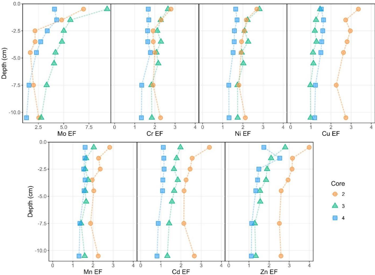
Figure 5: Vertical profiles of Cr, Mn, Ni, Cu, Zn, Mo and Cd enrichment factors (against Al) in cores 2, 3 and 4. Reference materials corresponds to the median values obtained on the Watringues marine plain soils (Sterckeman et al., 2004)
