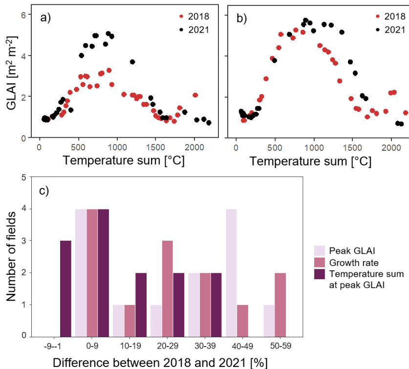
Fig. 4. Examples of temporal evolution of GLAI during 2018 (dry year) and 2021 (year with normal weather conditions) for two different fields with a) a large difference between the years and b) a small difference between the years. c) Number of fields by the percentage difference in crop growth proxies (i.e., peak GLAI, growth rate, and temperature sum at peak GLAI) between the years 2018 (dry year) and 2021 (year with normal weather conditions).
