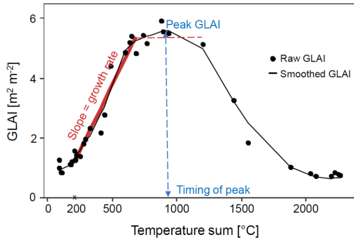
Fig. 3. Example from one of the fields showing the green leaf area index (GLAI) temporal development curve. We obtained proxies for the growth rate from the slope between a temperature sum of 200 °C until the start of the plateau (dashed red line), the peak GLAI from the maximum GLAI, and the timing of peak GLAI from the temperature sum at the peak GLAI. The raw GLAI values are shown by black dots and the smoothed GLAI is shown by the black curve.
