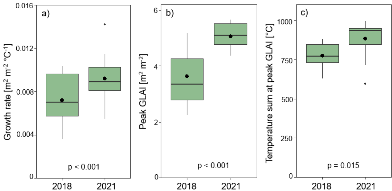
Fig. 5. Crop growth proxies obtained from the temporal evolution of green leaf area index (GLAI) in the dry year (2018) and the year with normal weather conditions (2021); a) growth rate, b) peak GLAI, and c) temperature sum at peak GLAI. Data show yearly average (black dots), median, upper and lower quartiles (box), and minimum and maximum values (whiskers). P-values from the t-test are displayed for the differences between the years (number of fields, n=13 ).
