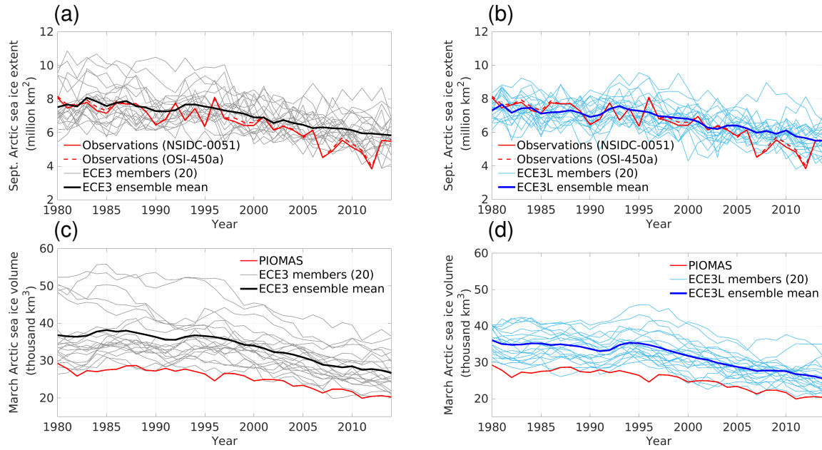
Figure 7. Arctic sea ice time evolution in the transient climate (1980–2014): (a) September extent ( SIC > 15\% ) ensemble of ECE3, (b) as in (a) but for ECE3L. Observations are from NSIDC with area pole-filling as well as OSI-450a. All are remapped to NSIDC-0051 grid. (c and d) as in (a and b) but for March volume (following the definition of the PIOMAS domain for areas thicker than 0.15 m).
