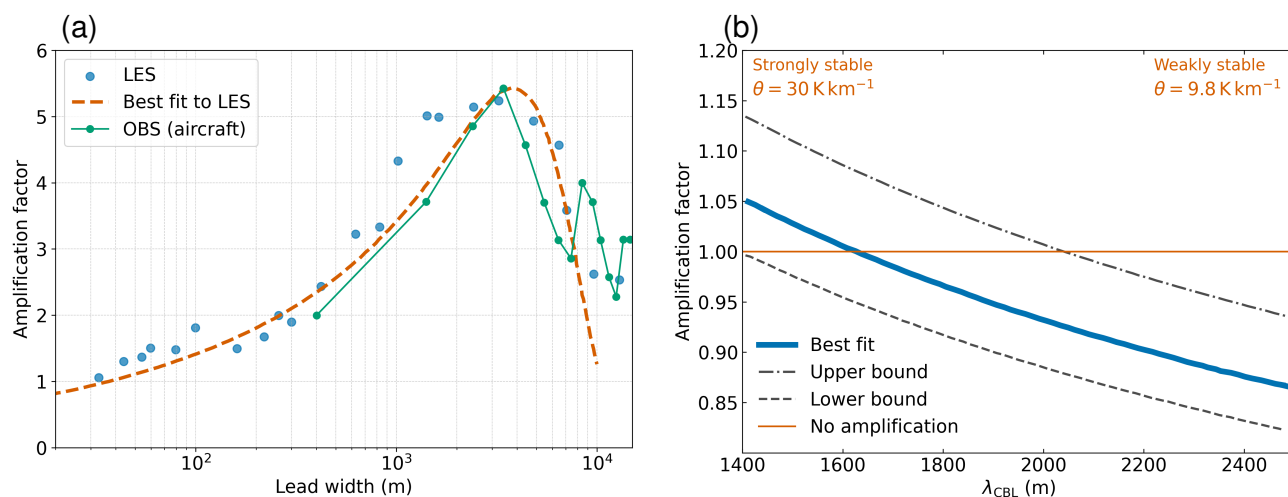
Figure A1. (a) Heat flux amplification factor (relative to open water) as a function of lead width, adapted from Esau (2007). Blue dots represent individual LES simulations, the red dashed line shows the best fit to LES data, and green dots indicate aircraft observations over the Baltic Sea. (b) Total sensible heat flux amplification across all leads. Panels (a) and (b) are adopted from Davy and Gao (2019) Figure 1 and 4, respectively.
