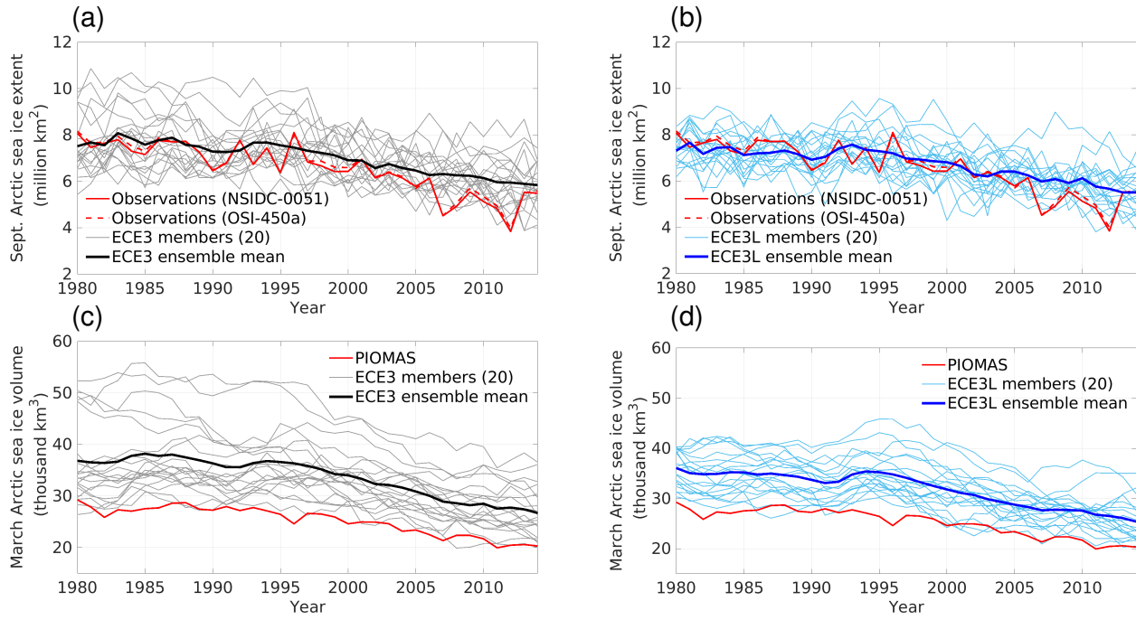
Figure 8. Arctic sea ice time evolution in the transient climate (1980–2014): (a) September extent ( \text{SIC} > 15\% ) ensemble of ECE3, (b) as in (a) but for ECE3L. Observations are from NSIDC with area pole-filling as well as OSI-450a. All are remapped to NSIDC-0051 grid. (c and d) as in (a and b) but for March volume (following the definition of the PIOMAS domain for areas thicker than 0.15 m).
