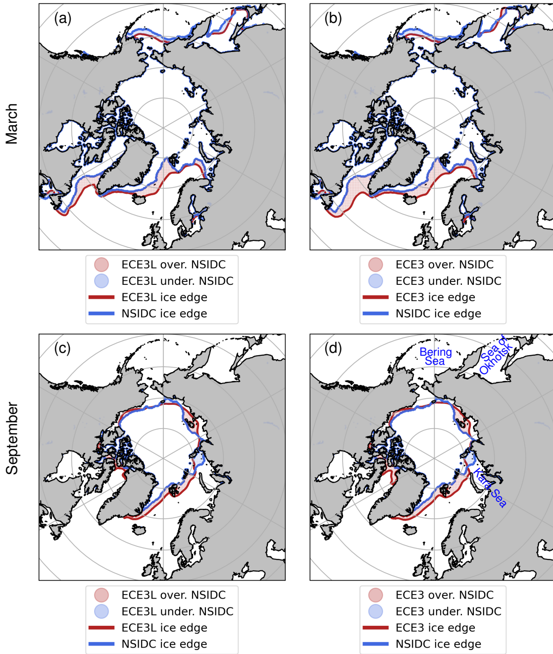
Figure 11. Integrated Ice Edge Error (IIEE, defined in Section 2.4) maps of ECE3L (a) and ECE3 (b) vs. NSIDC-0051 for March sea ice climatology (1980–2014). Red and blue indicate whether the model’s ensemble mean overestimates or underestimates the ice edge prescribed by NSIDC-0051, respectively. (c) and (d) as in (a) and (b), but for September sea ice. Sea ice edge is defined by the 15%-sea ice concentration contour.
