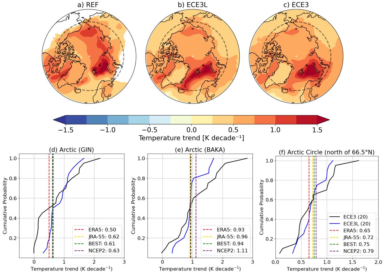
Figure 13. (a-c) Annual mean temperature trends for the transient climate (1980–2014), derived from the average of the observational datasets, ECE3L and ECE3. Areas without statistical significance are masked in panel (a), while panels (b) and (c) display significant trends across all areas. (d-f) Cumulative probability plots of temperature trend from ECE3 (black) and ECE3L (blue) ensembles for three regions: (d) the Greenland-Iceland-Norwegian Seas (GIN: 40^{\circ}\text{W} – 15^{\circ}\text{E} , 66.5^{\circ}\text{N} – 82^{\circ}\text{N} ), (e) the Barents and Kara Seas (BAKA: 15^{\circ}\text{E} – 100^{\circ}\text{E} , 70^{\circ}\text{N} – 82^{\circ}\text{N} ), and (f) the Arctic Circle. The locations of GIN and BAKA are shown in Fig. 1c. The grey dashed lines (a-c) depict the Arctic Circle ( 66.5^{\circ}\text{N} latitude). Observations are from ERA5, BEST, JRA-55 and NCEP2.
