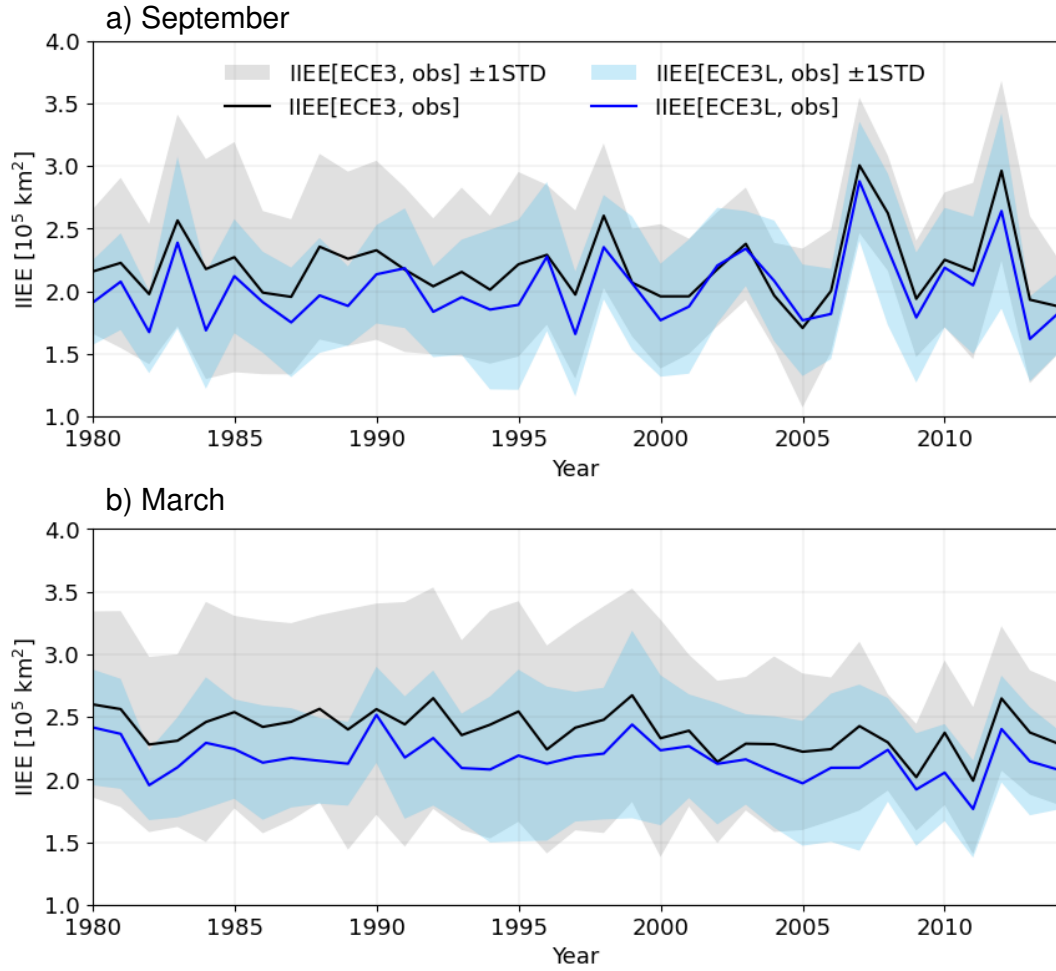
Figure 12. The time evolution of Integrated Ice Edge Error (IIEE) for September (a) and March (b) estimated for ECE3 (black) and ECE3L (blue) relative to NSIDC-0051 during the period 1980–2014: with ensemble means (thick line) and the model spread (the shaded area) indicated as one standard deviation from the mean across 20 members. Sea ice edge is defined by the 15%-sea ice concentration contour. Ensemble mean differences are statistically significant ( p < 0.05 , paired t -test); no trends are detected over time.
