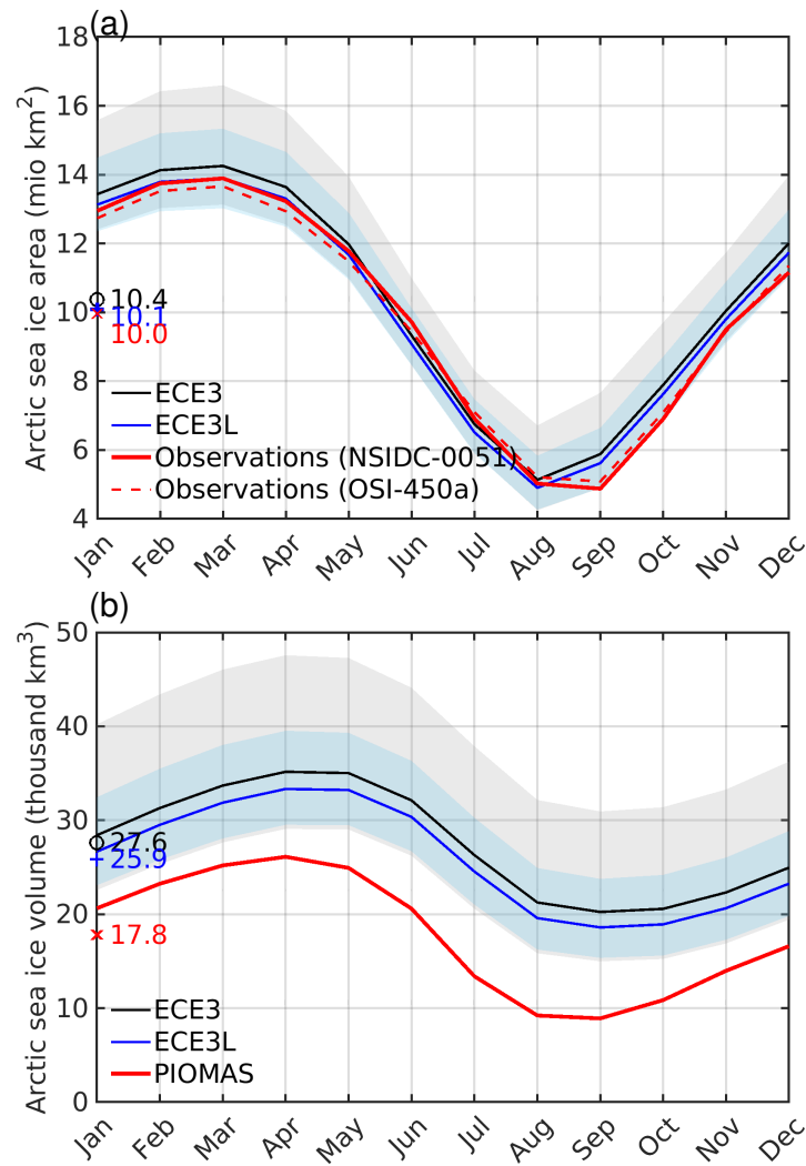
Figure 7. Comparison of annual cycle in the transient climate (1980–2014) between ECE3 (black) and ECE3L (blue) for (a) Arctic sea ice area and (b) Arctic sea ice volume. Thick lines represent the ensemble means, while the shaded areas indicate the spread between the 5th and 95th percentiles across 20 ensemble members, grey for ECE3 and light blue for ECE3L. Observations for the sea ice area include NSIDC and OSI-450a datasets, both remapped to the NSIDC-0051 grid. Sea ice volume is based on PIOMAS domain criteria (thickness > 0.15 m). The mean differences are statistically significant ( p < 0.05 , paired t -test).
