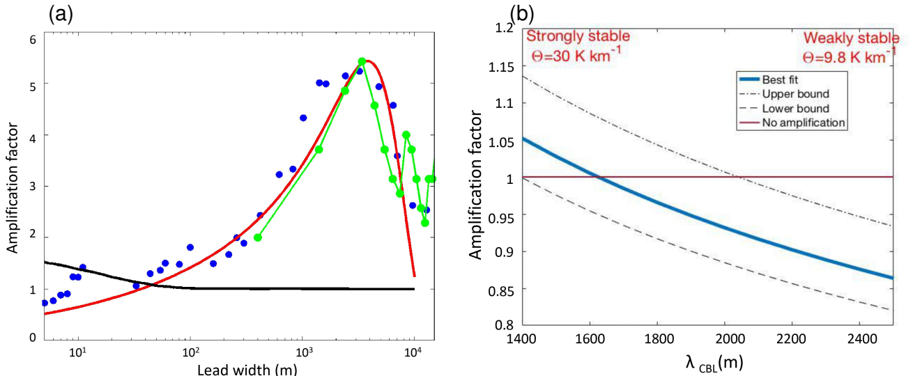
Figure A1. (a) Heat flux amplification factor (relative to open water) as a function of lead width, adapted from Esau (2007). Blue dots represent individual LES simulations, the thick red line shows the best fit to LES data, the black line represents parameterisation results from climate models, and green dots indicate aircraft observations over the Baltic Sea. (b) Total sensible heat flux amplification across all leads. Panels (a) and (b) are from Davy and Gao (2019) Figure 1 and 4, respectively.
