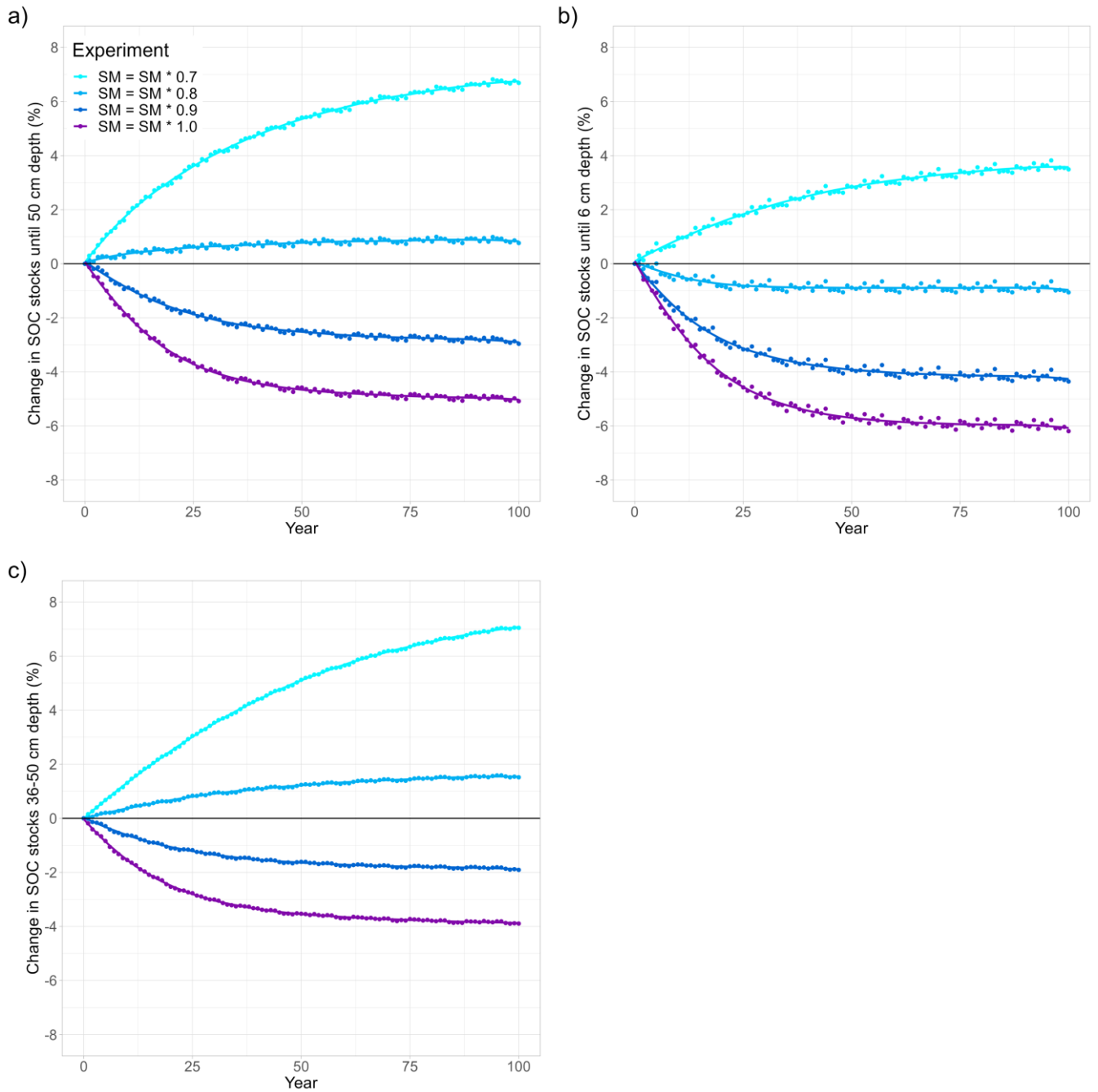
385 Figure 4: Soil moisture and temperature effects on long-term changes in modelled SOC stocks (% SOC lost since simulation year 0) in a) a whole soil column (0 - 50 cm), b) the topsoil layer (0 - 6 cm) and c) a subsoil layer (36 - 50 cm). In all model runs, the soil was warmed by 4.5 K. Soil moisture is reduced in 10% steps from ambient (SM * 1.0, purple) to 70% (SM * 0.7, light blue). In all runs, Q_{10,Km,X} = 1 (not temperature sensitive). The purple line (SM = SM * 1.0) is included from Fig. 3 for visual comparison.
