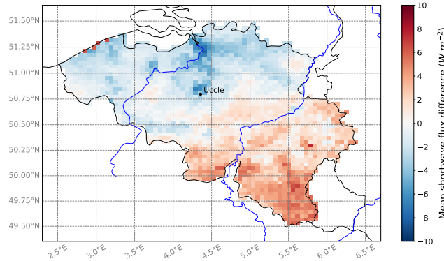
Figure 6. Mean shortwave flux differences of E7 (MAR v3.14 with ecRad and ecCKD) for 2011–2020. Grid-wide mean difference is +0.35 \text{ W m}^{-2} . Uccle location is given for Sect. 5.
