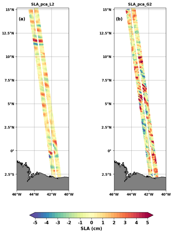
319 Figure 9: Snapshot of SWOT SLA_pca_L2 (a) and SLA_pca_G2 (b) on 08 April, 2023 (as in Figure 2). 320 SLA_pca_L2 is the sum of the SLAs of PCs less than or equal to 2 (PC1 and PC2). 321
