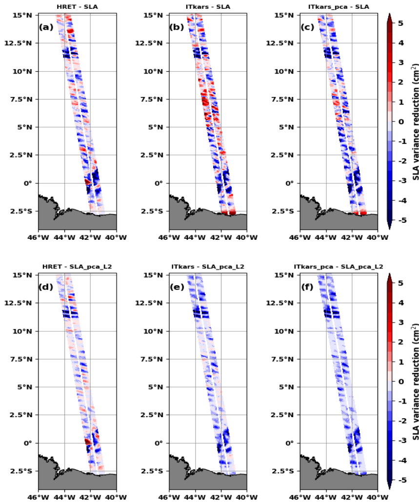
435 Figure 11: Variance reduction (in \text{cm}^2 ) on period 2 from early June to early July (last 34 cycles) when 436 using either M2 HRET (left column) or M2 ITkars_p1 (middle column) or M2 ITkars_pca_p1 (right 437 column) to correct the total SLA (top line) or SLA_pca_L2 (bottom line).
