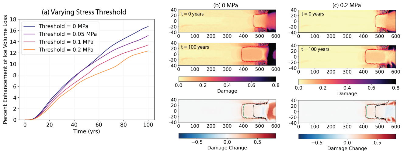
Figure 7. Effect of damage on ice volume loss for varying stress threshold: Results from a 100-year simulation for \sigma_t = 0, 0.2 MPa. (a) We show the percent enhancement of ice volume loss (difference in ice volume loss between a simulation with damage evolution and a simulation with damage initialization but no evolution as a percentage of total ice volume loss in the damage initialization simulation) and (b-c) the damage fields (initial and final damage, and total damage change) for \sigma_t = 0, 0.2 MPa.
