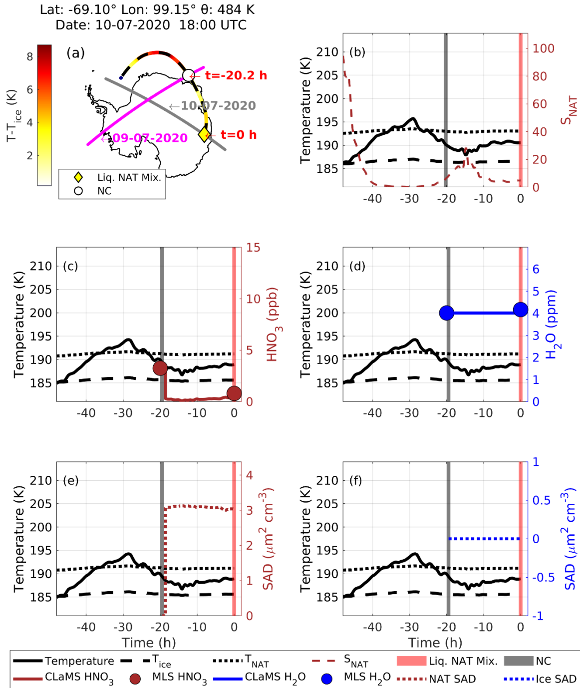
Figure 810. (a) The Lagrangian backward trajectory for a 48 h period starting at time, t = 0 h (corresponding to 18:00 UTC 10-07-2020). Here, the dashed black line is the backward trajectory and the color along this trajectory
