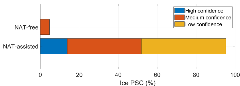
Figure 19. The percentage of ice PSCs formed via NAT-assisted and NAT-free nucleation processes, categorized by confidence levels based on backward trajectory observations and MLS HNO 3 availability. The bars represent high, medium, and low confidence cases for each process, with confidence levels determined by the presence of NAT and gas-phase HNO 3 concentrations along the trajectories.
