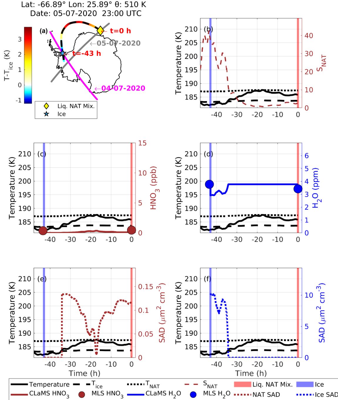
Figure 4011. Similar to Fig. 8-10 but for the Case no. 3-2 where ice preceded the liquid-NAT mixture along the Lagrangian backward trajectory.
