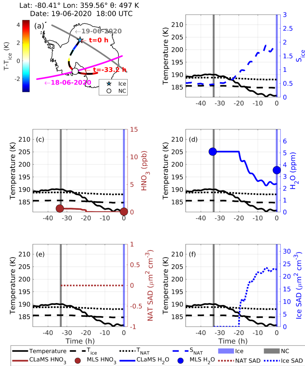
Figure 16. Same as Fig. 108 but for case no. 57 where ice nucleated without NAT.
