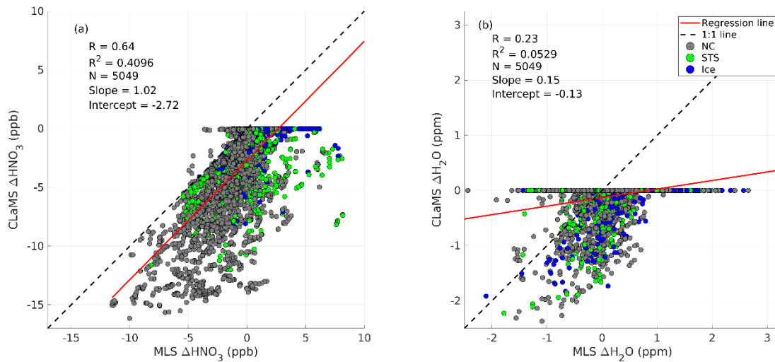
Figure 4213. (a) shows a scatter plot of MLS observed change ( \Delta ) in \text{HNO}_3 (ppb) against the CLaMS modeled change in \text{HNO}_3 (ppb), (b) shows a scatter plot of MLS observed change ( \Delta ) in \text{H}_2\text{O} (ppm) against the CLaMS modeled change in \text{H}_2\text{O} (ppm). The dashed line represents a 1:1 fit, and the solid red line represents the linear regression line. Here, ‘R’ is the correlation coefficient, ‘ R^2 ’ is the correlation of determination, and N is the total number of data points used. The color of the circles corresponds to each PSC type preceding to liquid-NAT mixture along the backward trajectory. Grey for NC, green for STS, and blue for ice PSC.
