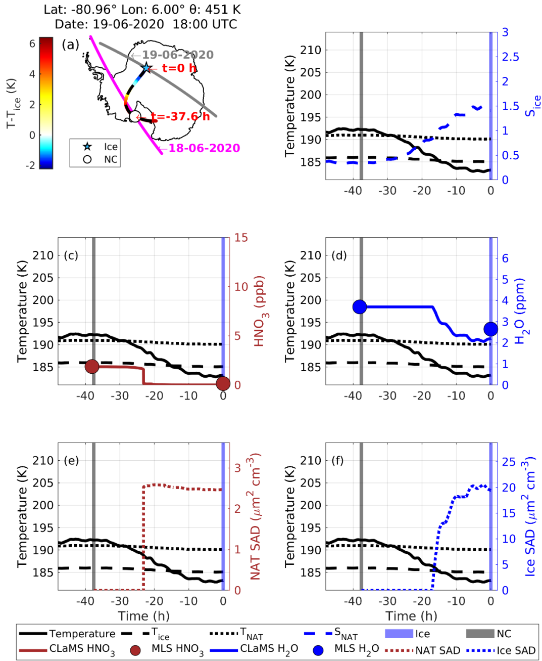
Figure 15. Same as Fig. 108 but for case no. 64 where ice nucleation on NAT is shown.
