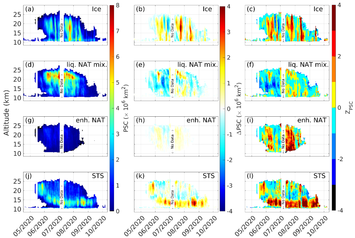
Figure 76: CALIPSO Antarctic PSC monthly mean areal coverage (left column, panels a, d, g, and j), anomaly (middle column, panels b, e, h, and k), and standardized anomaly (right column, panels c, f, i, and l) for the year 2020. Here, 'liq. NAT mix.' is a liquid-NAT mixture and enh. NAT is enhanced NAT.
