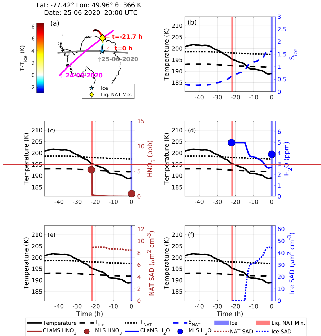
Figure 14. Same as Fig. 8 but for case no. 5 where ice nucleation on NAT is shown.
