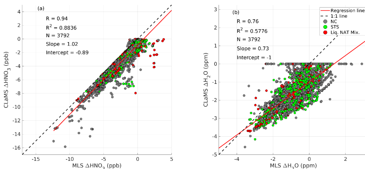
Figure 18. Same as Fig. 12.13. But for the case of ice formation.
