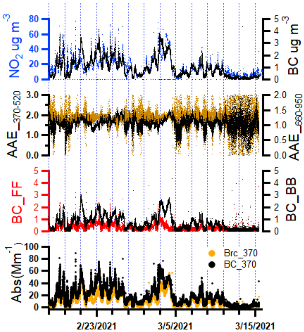
Figure S3. Overview of NO 2 and black carbon (BC), absorption Ångström exponents (AAE) at 370 to 520 nm (AAE 370-520 ), AAE at 660 to 950 (AAE 660-950 ), BC_FF, BC_BB, Abs 370 of BrC, and Abs 370 of BC.
