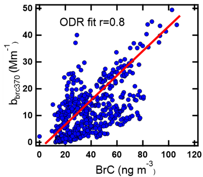
Figure S6. The correlation of BrC mass and absorption ( b_{\text{brc}370} ).
