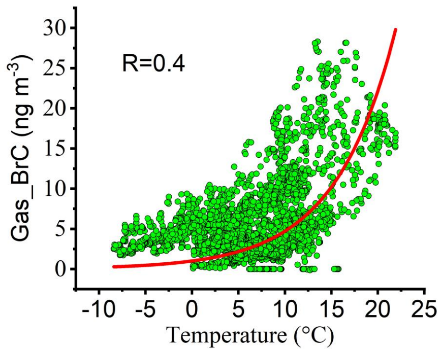
Figure S8. The correlation of gas-phase BrC and temperature based on exponential fit ( y=e^{(0.15*x)} )
