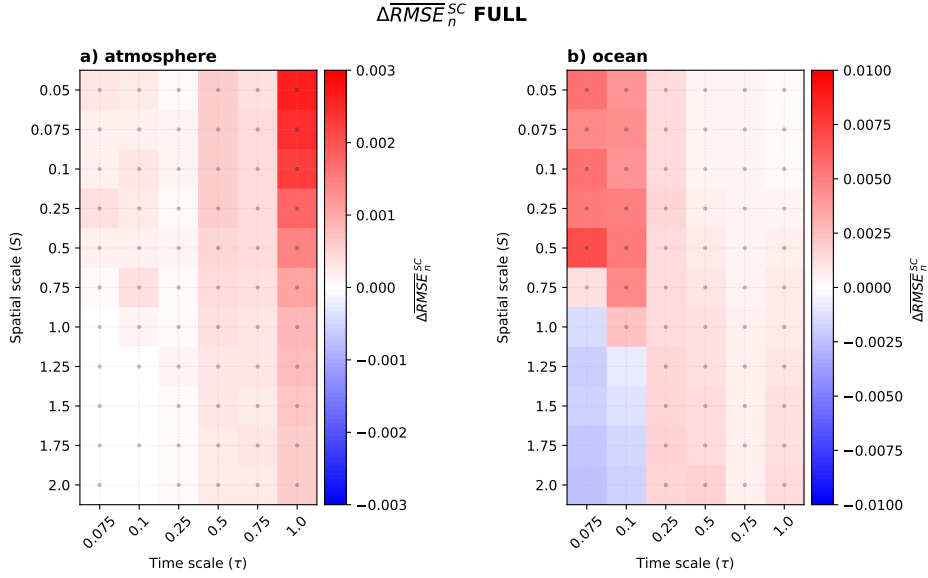
Figure 10. FULL experiment \Delta \overline{RMSE}_n^{SC} for a) atmosphere and b) ocean. The colour red (blue) indicates that the SC error is larger (smaller) than that of the WC experiments. Dotted area indicates \Delta \overline{RMSE}_n^{SC} \geq 0 , meaning that SCDA degrades over WCDA. Note that the colourbar for both components has different limits.
