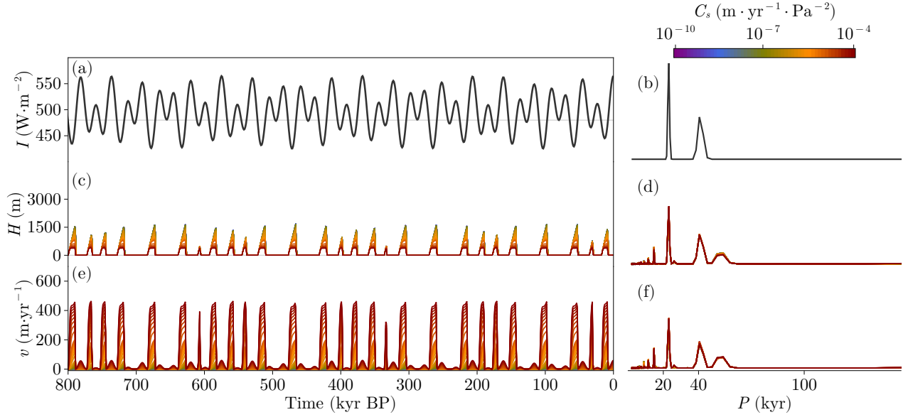
Figure 3. Results of the LIN simulation. (a, c, e) Time series obtained from the model using different sliding factors C_s . (b, d, f) Normalized periodograms obtained from the time series in the left column. Note that when normalizing spectra, series were cut off for periods larger than 200 kyr.
