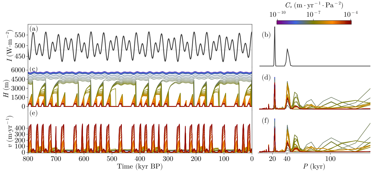
Figure 7. Results from the ISOS simulation. (a, c, e) Time series obtained from the model using different sliding factors C_s and (b, d, f) associated normalized periodograms. Note that when normalizing spectra, series were cut off for periods larger than 200 kyr.
