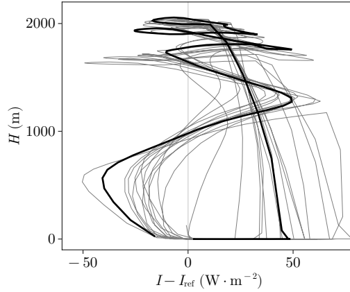
Figure 17. Trajectories of the AGING experiment with \tau_\alpha = 50 kyr and C_s = 0.3 \cdot 10^{-8} \text{ m yr}^{-1} \text{ Pa}^{-2} . We highlight the last glacial cycle in black.
