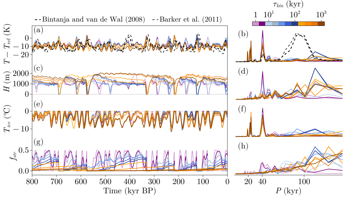
Figure 13. Results of the THERM simulation using C_s = 5 \cdot 10^{-6} \text{ m yr}^{-1} \text{ Pa}^{-2} . (a, c, e, g) Time series obtained from the model using different \tau_{kin} (colors). (b, d, f, h) Normalized periodograms obtained from the time series in the left column. Note that when normalizing spectra, series were cut off for periods larger than 200 kyr.
