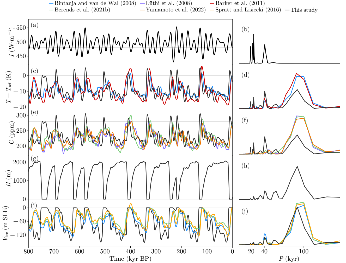
Figure 16. Results of AGING simulation (black) for \tau_\alpha = 50 kyr and C_s = 0.3 \cdot 10^{-7} \text{ m yr}^{-1} \text{ Pa}^{-2} (in comparison with Bintanja and Van de Wal, 2008; Lüthi et al., 2008; Barker et al., 2011; Spratt and Lisiecki, 2016; Berends et al., 2021b; Yamamoto et al., 2022). Note that the initial conditions are applied at 1000 kyr BP just to let the model equilibrate.
