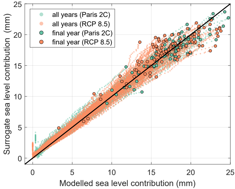
Figure E1. Cumulative sea level contribution from the ASE for each year, between 2021-2100, as predicted for the test subset of \hat{U}a-fwd simulations and the LSTM surrogate model. The cumulative sea level contribution for the final year of each simulation, which make up the bulk of our uncertainty quantification and analysis, are highlighted with a black edge.
