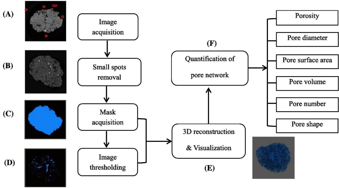
Fig. 3. Procedures used for the visualization and quantification of soil aggregate pore networks.
