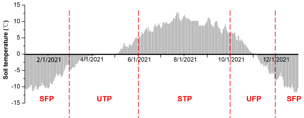
Fig. 2. Daily average soil temperature in 2021 and the classification of freeze–thaw stages (SFP–stable frozen period, UTP–unstable thawing period, STP–stable thawed period and UFP–unstable freezing period).
