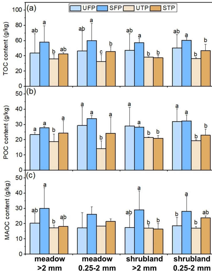
Fig. 6. Changes of SOC content (a-TOC, b-POC and c-MAOC) of soil aggregates during the seasonal FT process. Bars represent the mean \pm standard error (n=9). Different lowercase letters denote significant differences among SOC contents in different FT periods ( p < 0.05 ).
