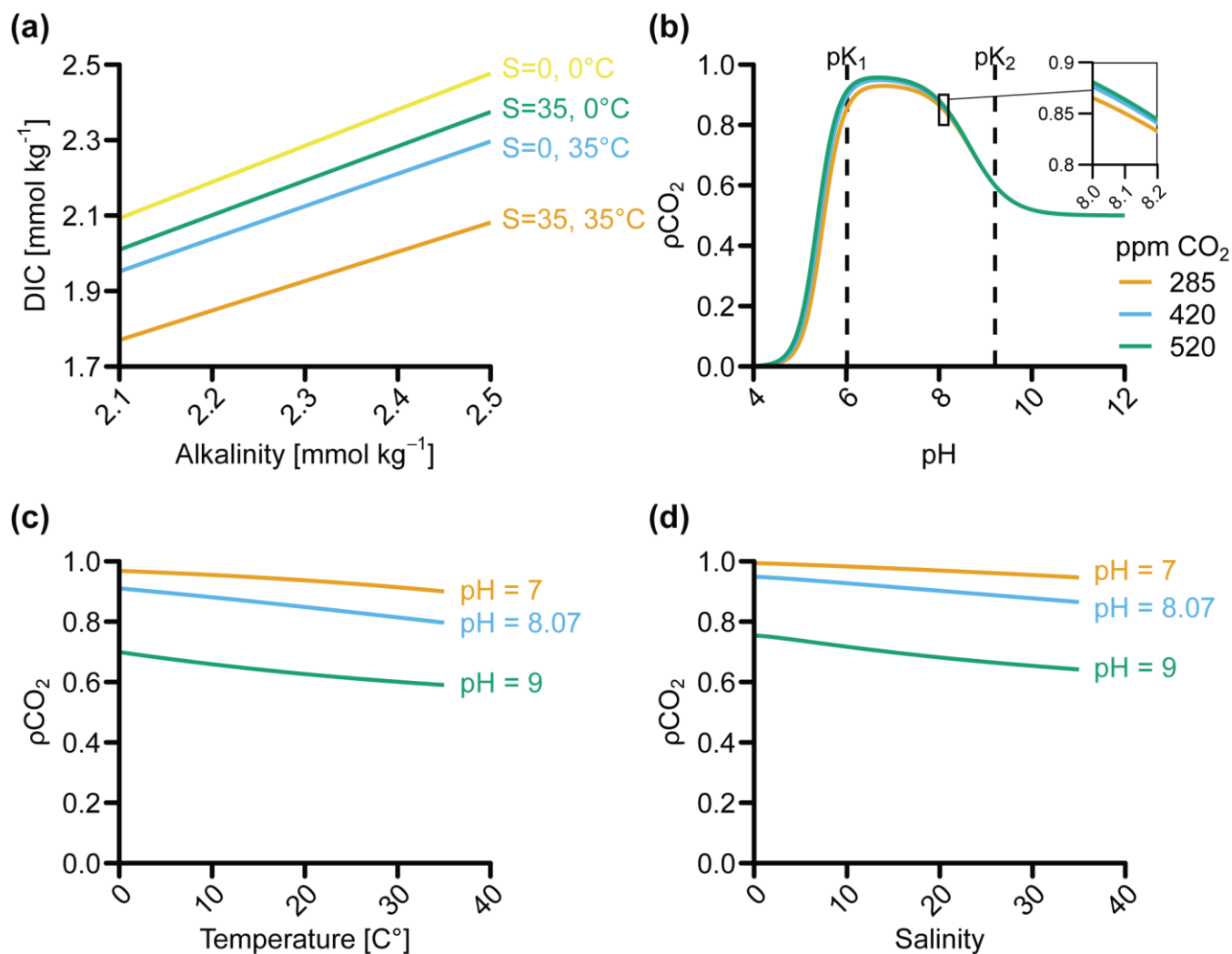
810 Figure 6. The CO 2 sequestration efficiency ( \rho_{CO_2} ) as a function of environmental parameters (unless otherwise stated pH = 8.07, temperature = 15 °C, salinity = 35, f_{CO_2} = 420 ppm). (a) Predicted DIC as a function of alkalinity for a set of endmember temperature and salinity values. (b) \rho_{CO_2} as a function of pH at different levels of atmospheric CO 2 (constant temperature and salinity), with pK values from Lueker et al. (2000). Typical seawater pH is shown in magnification. (c) \rho_{CO_2} as a function of temperature at different pH levels (constant salinity and f_{CO_2} ).
