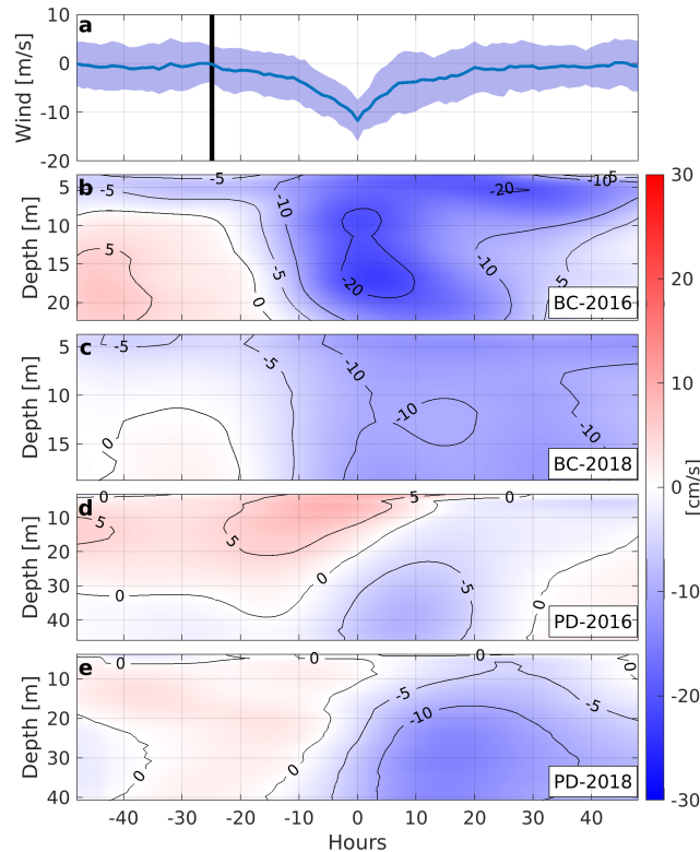
Figure 10. Composite time series of (a) meridional wind in Punta Hualpén and its standard deviation. The black vertical line shows the onset of the average time at which an extratropical cyclone appears in the detection area before t_0 . Composite currents for (b) BC2016, (c) BC2018, (d) PD2016, and (e) PD2018 along the axis shown in figure 1
