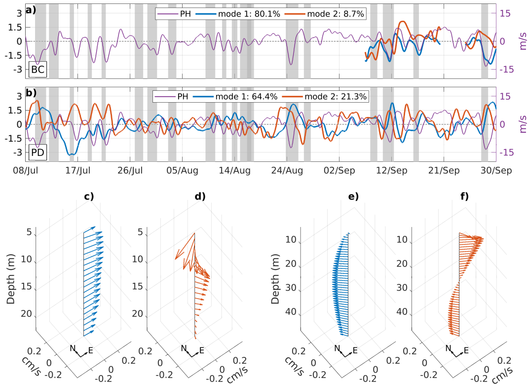
Figure 6. Meridional wind from PH Punta Hualpén Station (in purple) and time series of modes 1 (blue) and 2 (red) during 2016 for (a) BC and (b) PD. Vertical structures of the respective modes at (c-d) BC and (e-f) PD.
