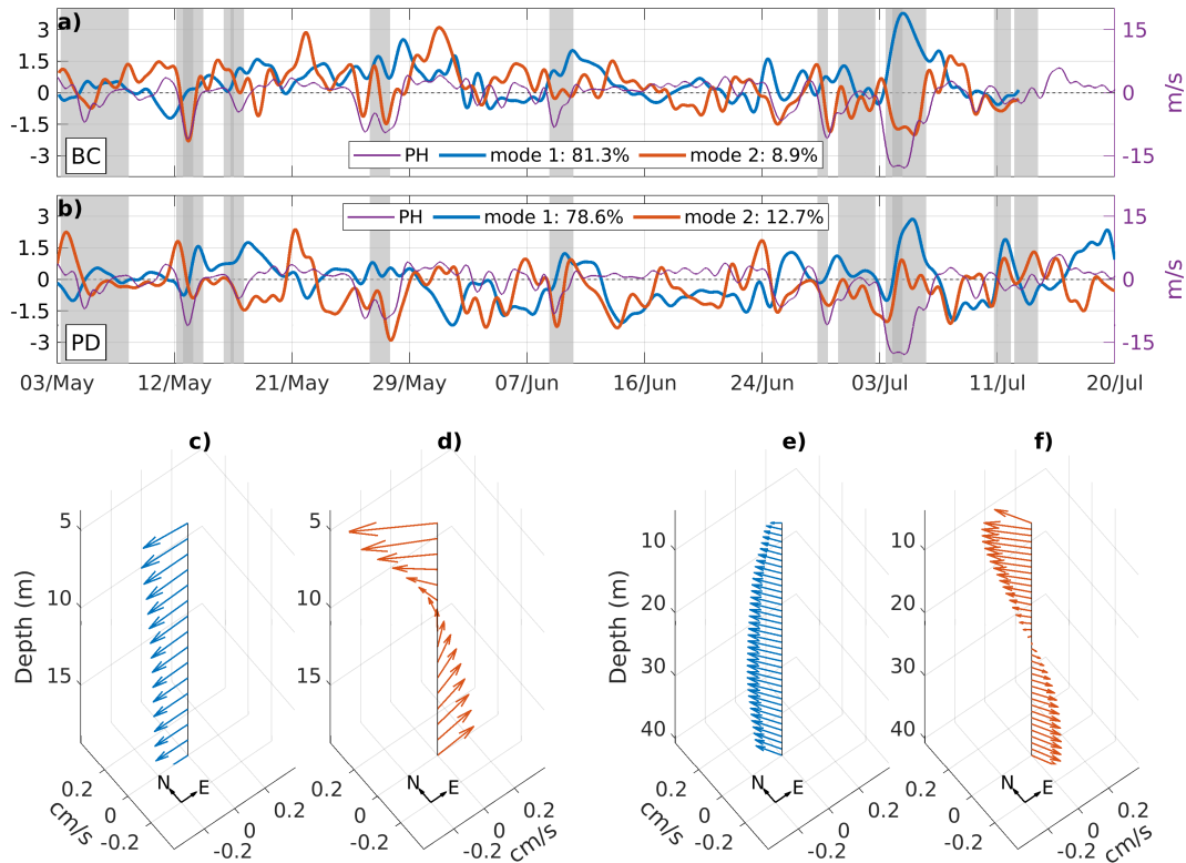
Figure 7. Meridional wind from PH Punta Hualpén Station (in purple) and time series of modes 1 (blue) and 2 (red) during 2018 for (a) BC and (b) PD. Vertical structures of the respective modes at (c-d) BC and (e-f) PD.
