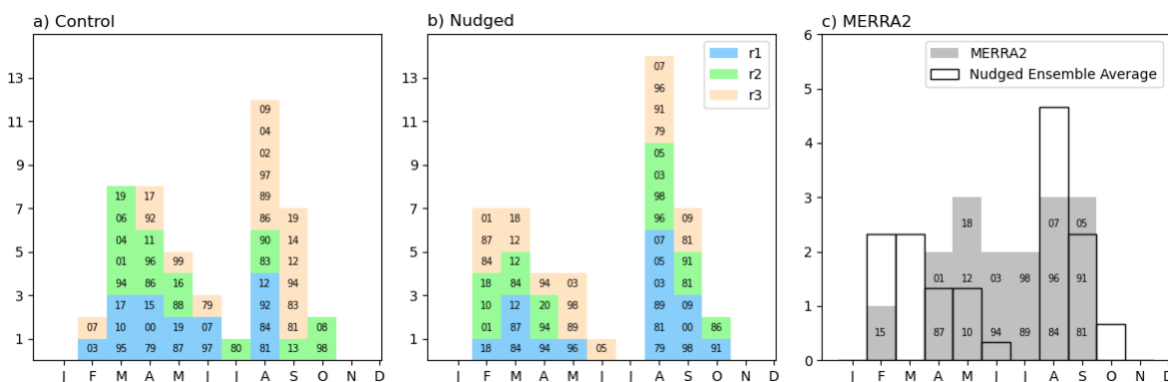
Figure 2: Histogram of QBOE to QBOW phase transition months at 5hPa for the (a) Control and (b) Nudged ensemble members and (c) at 10 hPa for MERRA-2. Corresponding years for the (a) Control and (b) Nudged and (c) MERRA-2 are listed. In figures a-b the colours denote the different ensemble-members. Averages of the three Nudged run ensemble members are overlaid in (c).
