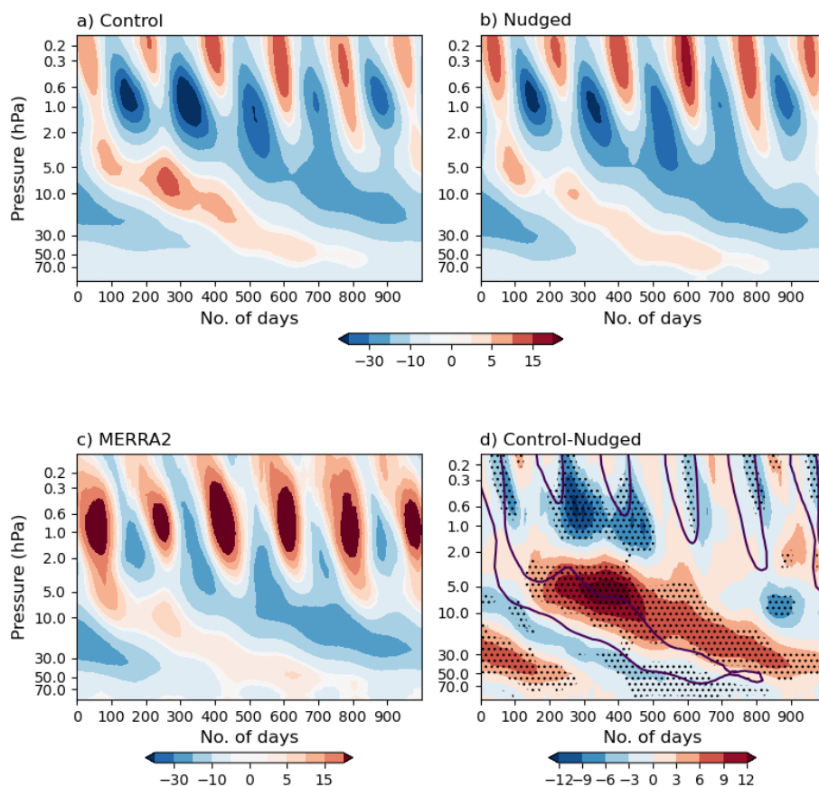
Figure 3: QBO composite of zonal-mean zonal wind (m/s) for the (a) Control experiment, (b) Nudged experiment and (c) MERRA-2. The composite members start from 1 st of March or 1 st of September whichever is closest to the start of the QBOW phase. The 5hPa reference level is used to identify the start of the QBO westerly phase in model and 10 hPa is used in MERRA2 (see text for more details). (d) Difference between the Control and Nudged experiments, with the QBO composite winds from the Control experiment overlaid as black contours. Stippling denotes 95% confidence interval. Stippling denotes 95% confidence interval.
