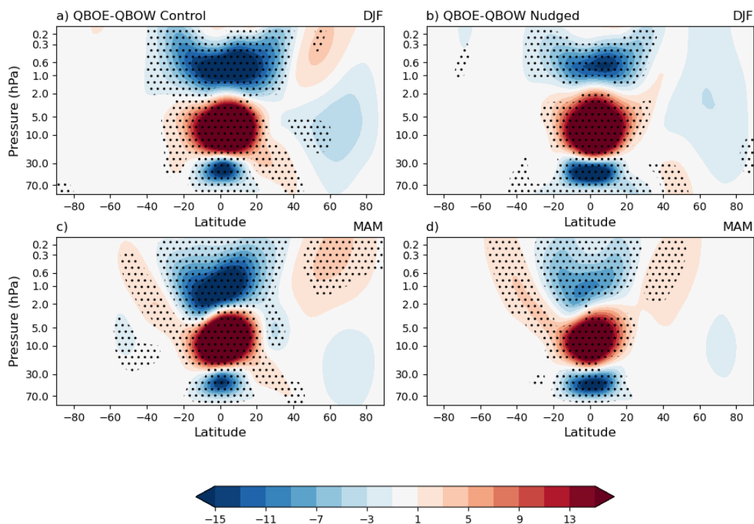
325 Figure 4: Latitude-height seasonal composites of QBOE minus QBOW zonal-mean zonal winds (m/s) from a) Control experiment DJF, b) Nudged experiment DJF, c) Control experiment MAM and d) Nudged experiment MAM. The phase of the QBO has been defined at 50 hPa. Stippling denotes at 95% confidence interval.
