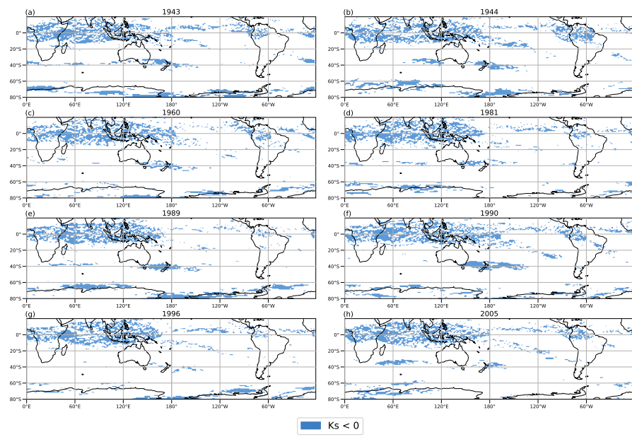
Figure S2: Stationary wave number K_s fields for each negative IOD event in the period 1940-2020.
