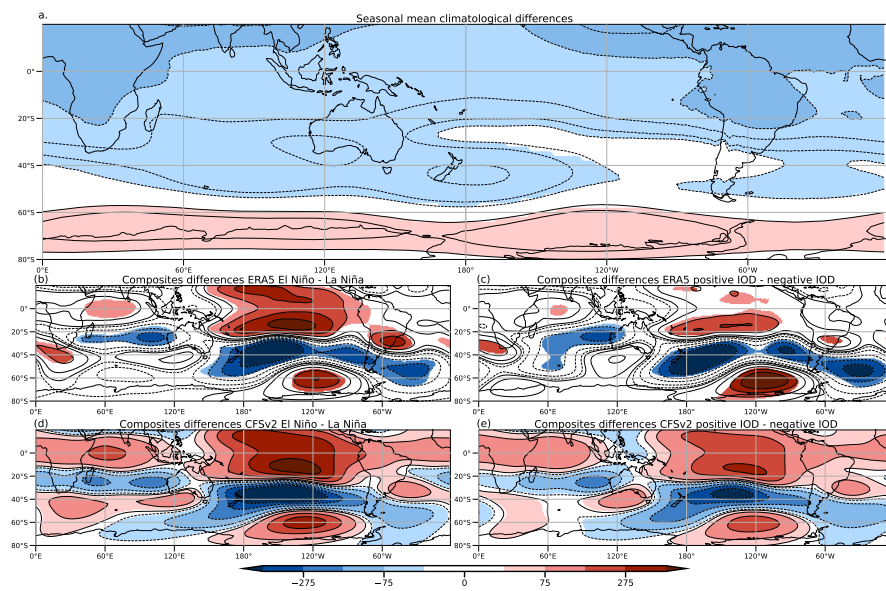
Figure S3: (a) Differences in the mean field of geopotential height (m) at 200hPa between CFSv2 and the ERA5 model in SON for 1982-2020 period. Differences between the mean fields of geopotential height anomalies (m) at 200hPa between the positive and negative phases of the ENSO (b, d) and IOD (c, e) events for ERA5 (b, c) and CFSv2 (d, e).
