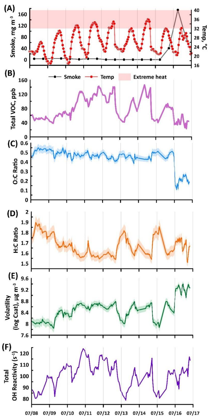
475 Figure 6. (A) Time series profile of the smoke, and temperature observed at MOFLUX, (B) sum of VOC mixing ratio, 476 (C) weighted O:C, (D) H:C ratios, (E) volatility, and (F) total reactivity during the intensive operational period 477 between July 8 to 17. The shaded regions of O:C, H:C, and volatility are the weighted standard deviations.
