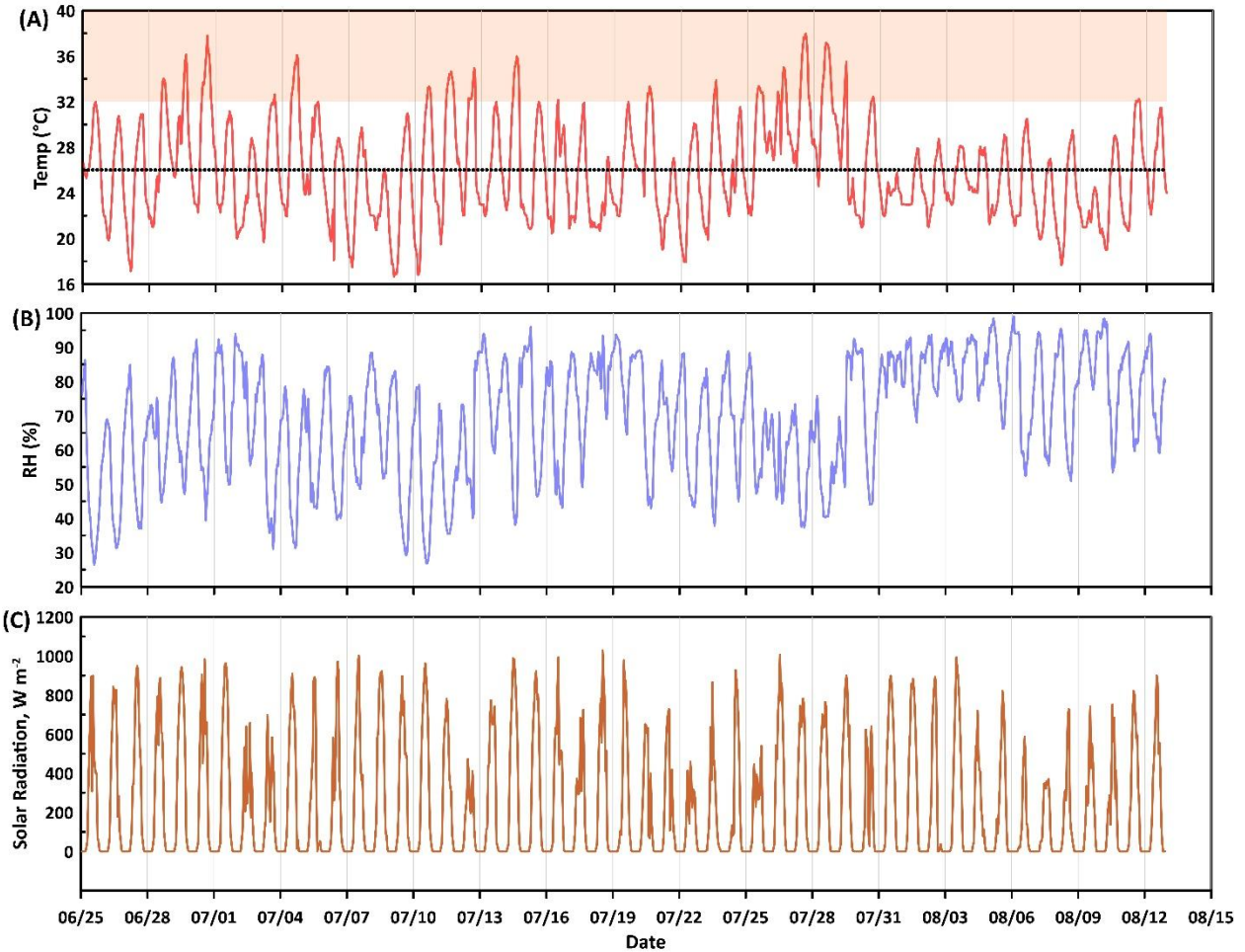
Figure 1. Time series profile of (A) temperature, (B) relative humidity, RH, and (C) downward solar radiation at the temperate mixed deciduous forest in Missouri. The dotted line in the temperature plot is the average value during the measurement duration, and the shaded filled area denotes the extreme temperature conditions ( >32^{\circ}\text{C} ).
