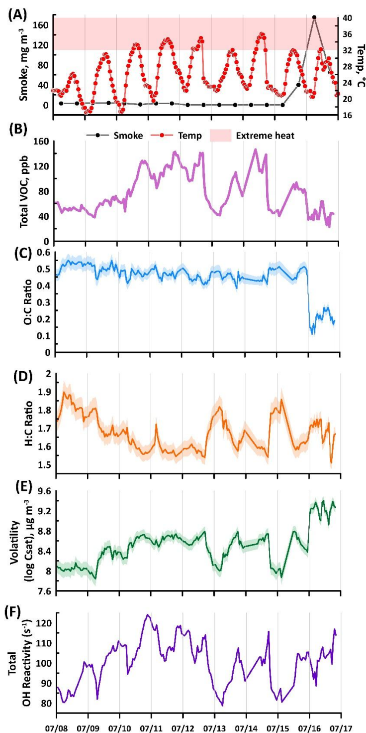
Figure 5. (A) Time series profile of the smoke, and temperature observed at MOFLUX, (B) sum of VOC mixing ratio, (C) weighted O:C, (D) H:C ratios, (E) volatility, and (F) total reactivity during the intensive operational period between July 8 to 17. The shaded regions of O:C, H:C, and volatility are the weighted standard deviations.
