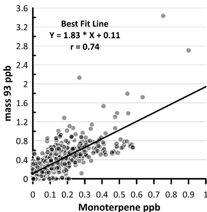
Fig S4: Correlation plot of mass 93 and monoterpene at mass 137.
