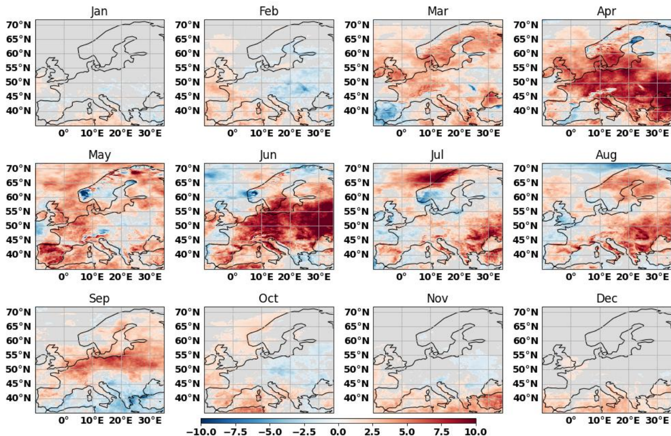
205 Figure 3: The spatial trends in SIS (in W/m 2 /decade) based on the CLARA-A3 CDR (1982-2020). Only those trends that are significant at 90% confidence interval are shown.
